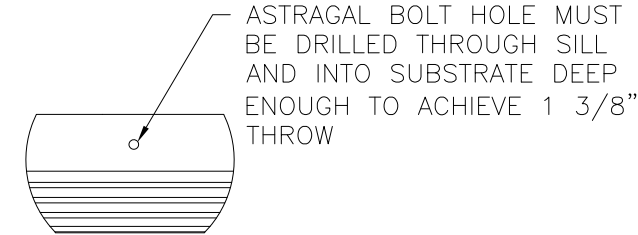
ASTRAGAL SILL DETAIL
