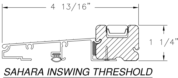
STANDARD INSWING THRESHOLD
