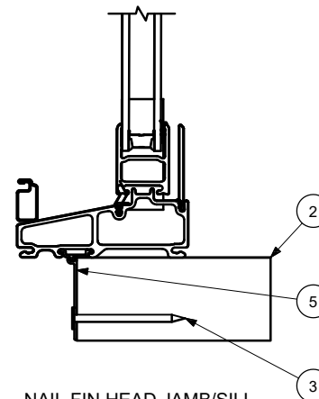
NAIL FIN HEAD JAMB/SILL SCALE 1:2
