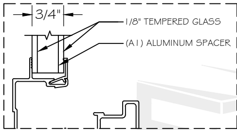
(G1) GLASS DETAIL (NON IMPACT)
