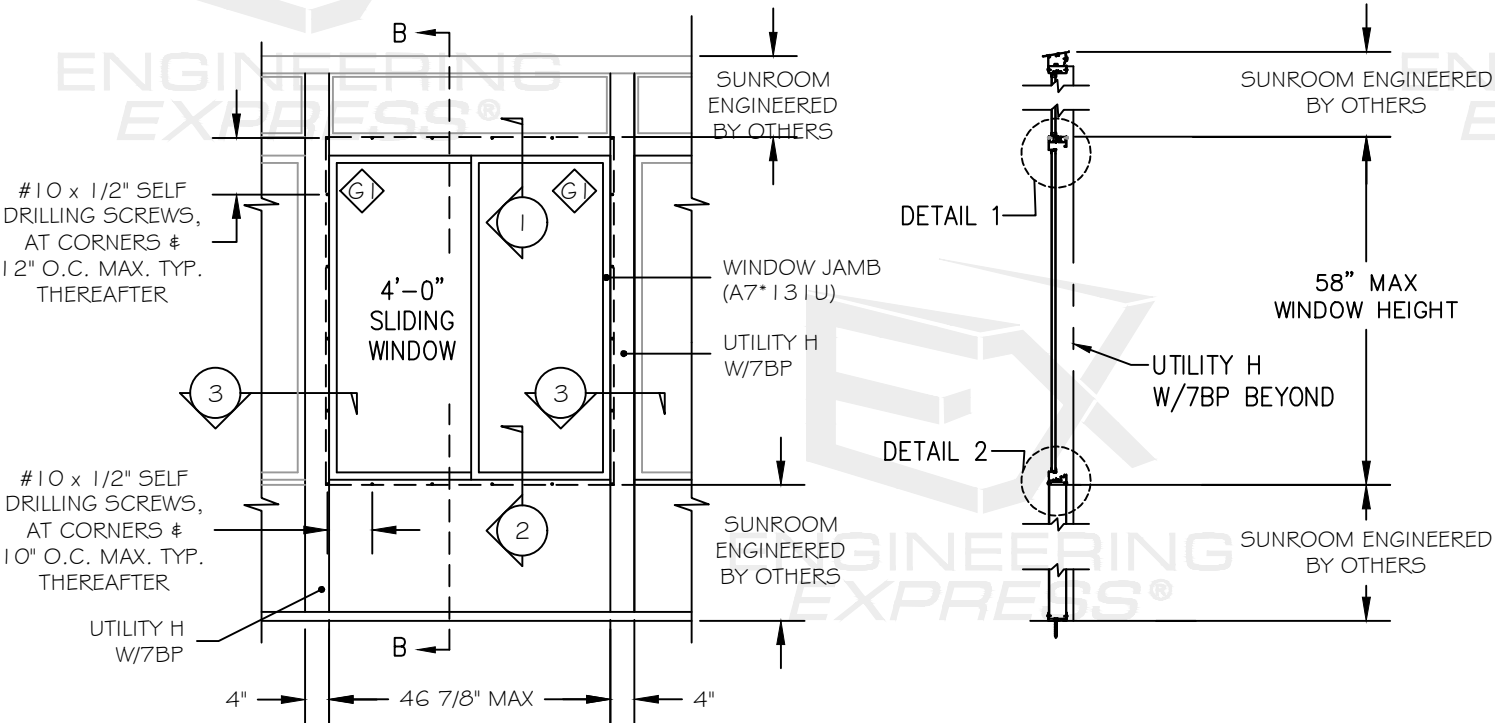
(A) TYP. ELEVATION SCALE: NTS
