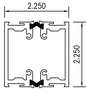
43 MULLION FRAME
