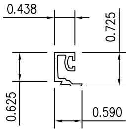
8 1" GLASS STOP
