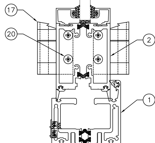
E 7 VERTICAL CROSS SECTION OUTFOLD
