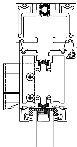
SLIDE-IN DOOR STOP (52262) WITH COEX BULB GASKET (GA000022-00-02) ATTACHED WITH #6 X 1" C.S. S.M.S. (FA000085-00-00) 3" IN FROM ENDS & 8" O.C. DOOR ADAPTER (40921)
