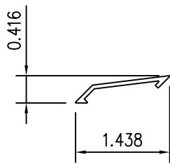
15 5 1/4" HINGE COVER
