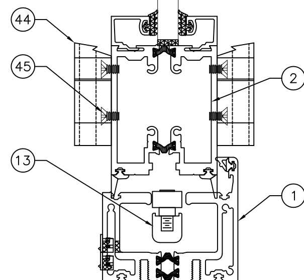
F 7 VERTICAL CROSS SECTION OUTFOLD TOP LOAD
