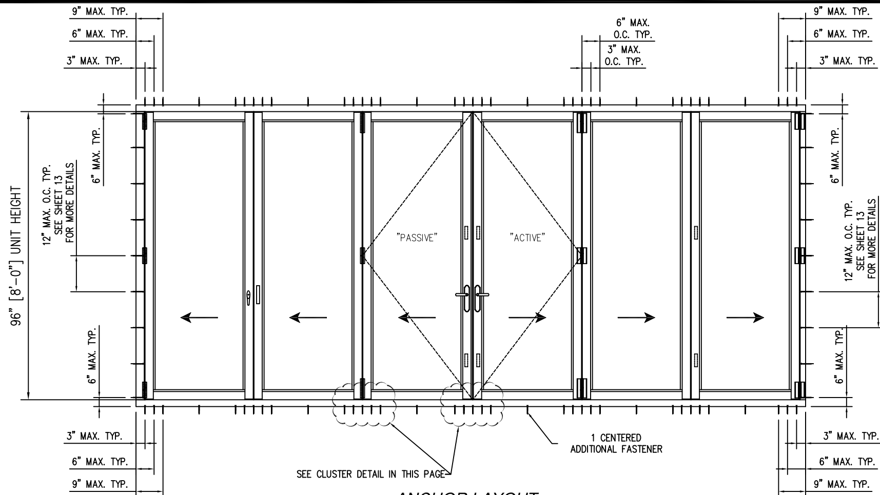
ANCHOR LAYOUT APPLICABLE TO ALL CONFIGURATIONS.
