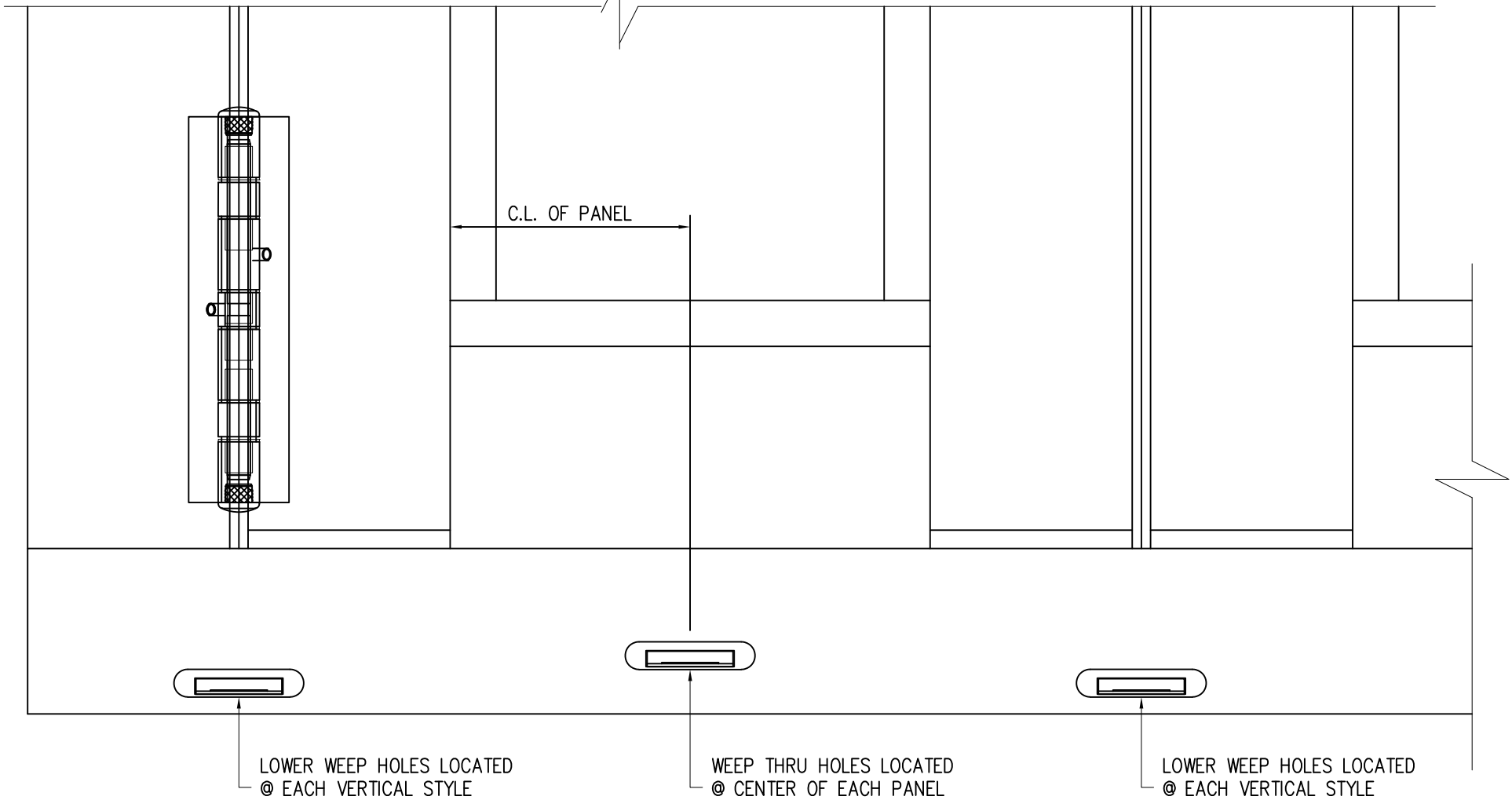
WEEP LOCATIONS
