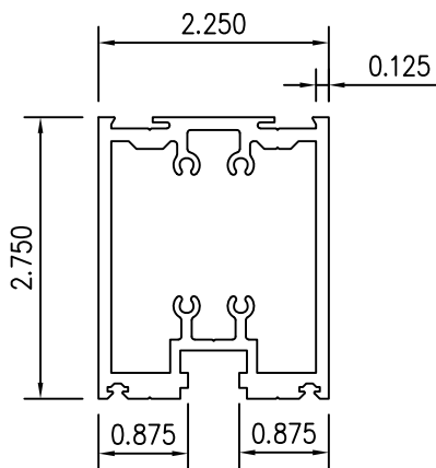
NON-THERMAL FRAME
