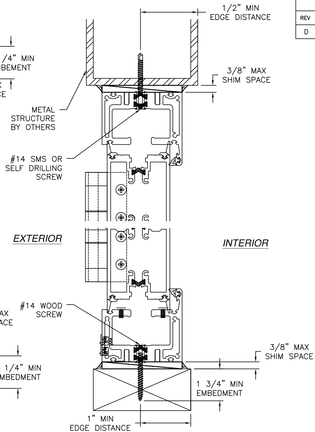
VERTICAL CROSS SECTION WOOD FRAMING OR 2X BUCK OR METAL STRUCTURE INSTALLATION STANDARD SILL SHOWN FLUSH SILL SIMILAR
