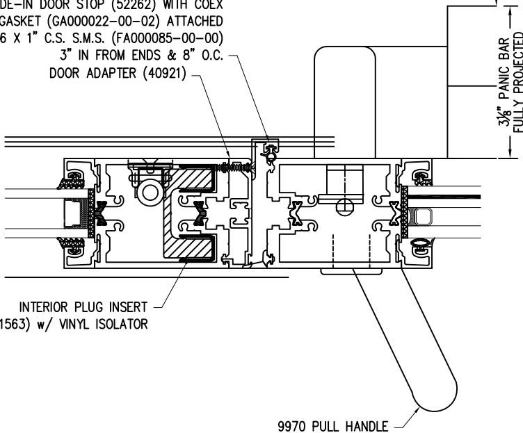
9970 PULL HANDLE
