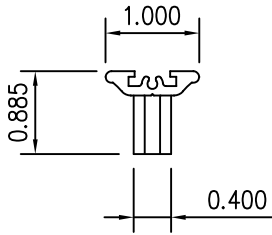
6 LOW-PROFILE HANDLE
