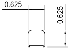
13 IDLER BODY
