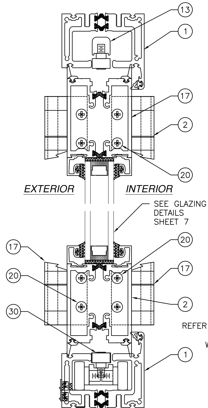
C 6 VERTICAL CROSS SECTION OUTFOLD BOTTOM LOAD
