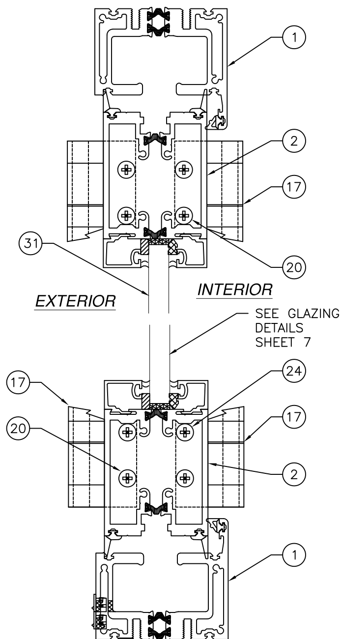
B 6 VERTICAL CROSS SECTION OUTFOLD
