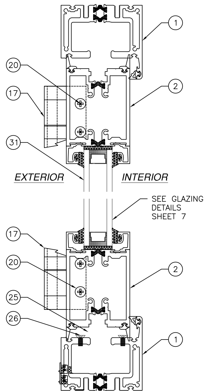
A 6 VERTICAL CROSS SECTION OUTFOLD
