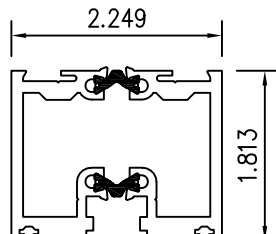
18 FRAME NARROW
