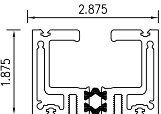
48 FLUSH SILL
