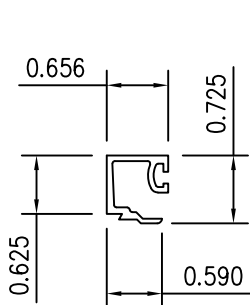
9 9/16" GLASS STOP
