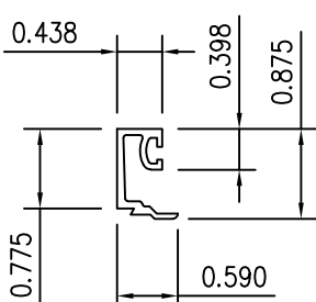
1/2" GLASS STOP
