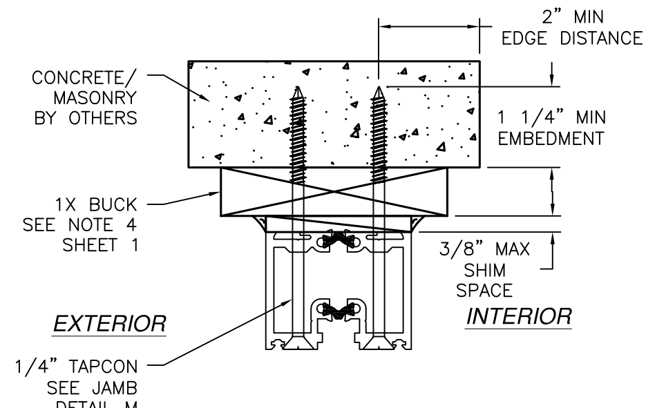
JAMB INSTALLATION DETAIL CONCRETE/MASONRY S47543 NO REINFORCEMENT
