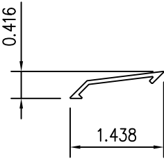
15 5 1/4" HINGE COVER
