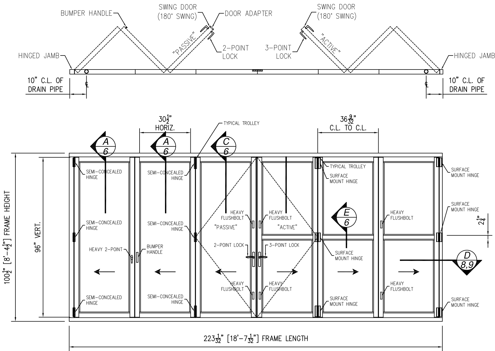
SERIES SI3000 FGW 3X8 PANEL INFOLD ALUMINUM REINFORCED EXTERIOR VIEW UNLIMITED NUMBER OF PANELS IN UNLIMITED CONFIGURATION ARE APPROVED AS LONG AS INDIVIDUAL PANEL AREA DOES NOT EXCEED 24.06 FT² AND USES VERTICAL CONDITIONS AS SHOWN.
