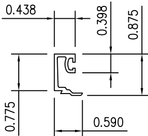
1/2" GLASS STOP
