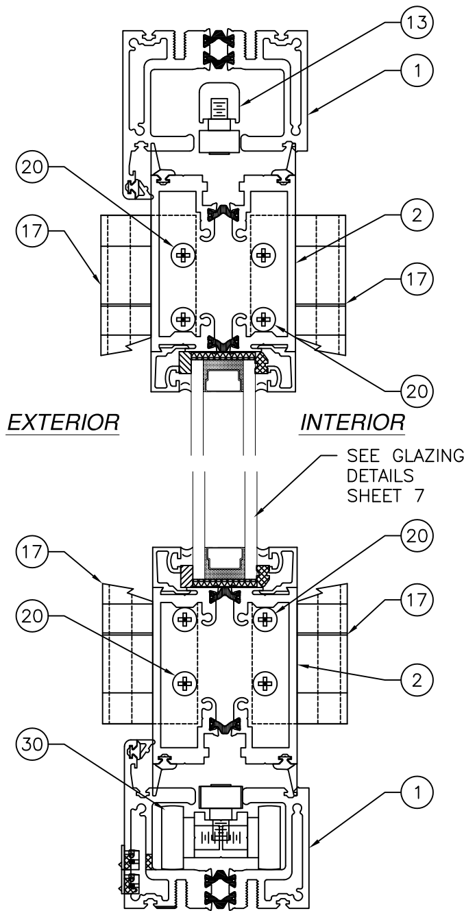
C 6 VERTICAL CROSS SECTION BOTTOM LOAD
