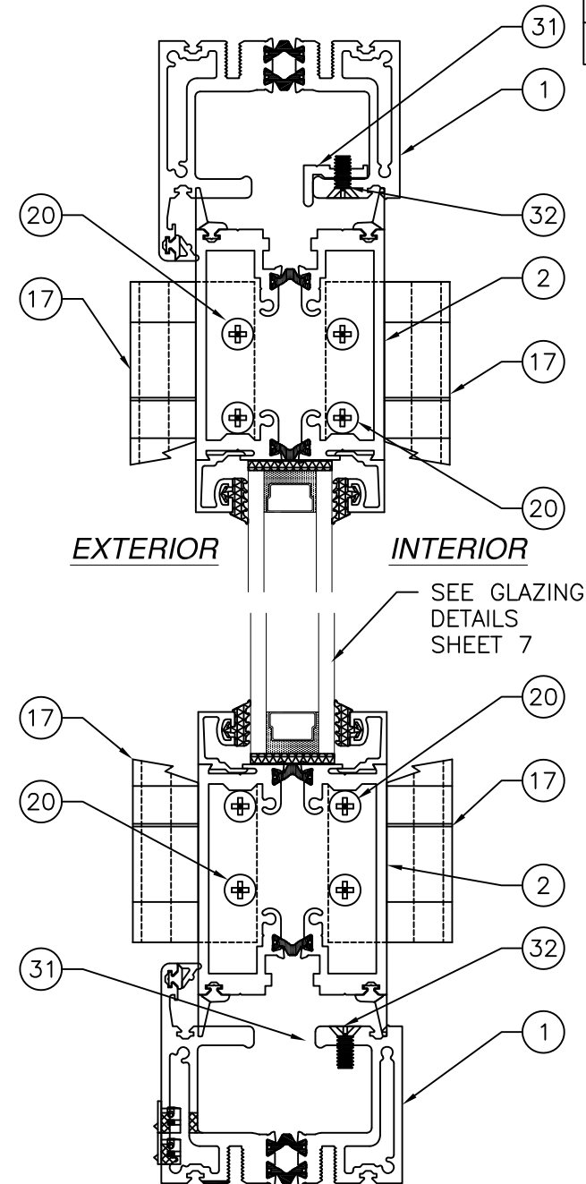
B 6 VERTICAL CROSS SECTION
