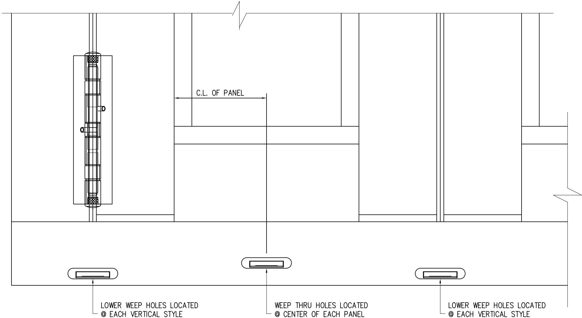
WEEP LOCATIONS
