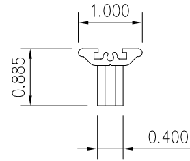
6 LOW-PROFILE HANDLE
