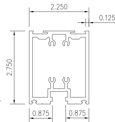
NON-THERMAL FRAME
