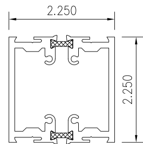
43 MULLION FRAME
