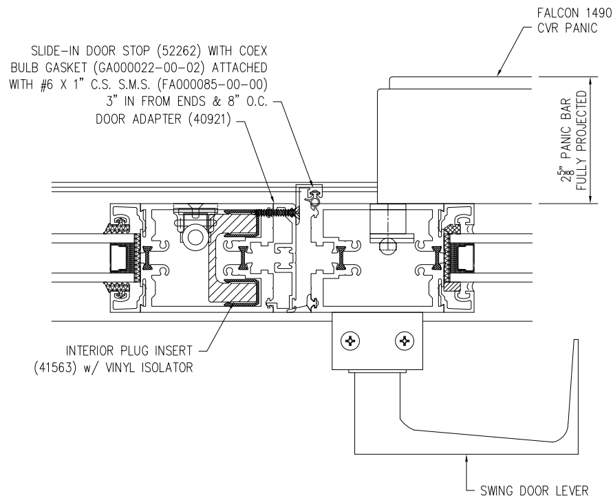
PANIC BAR DETAILS
