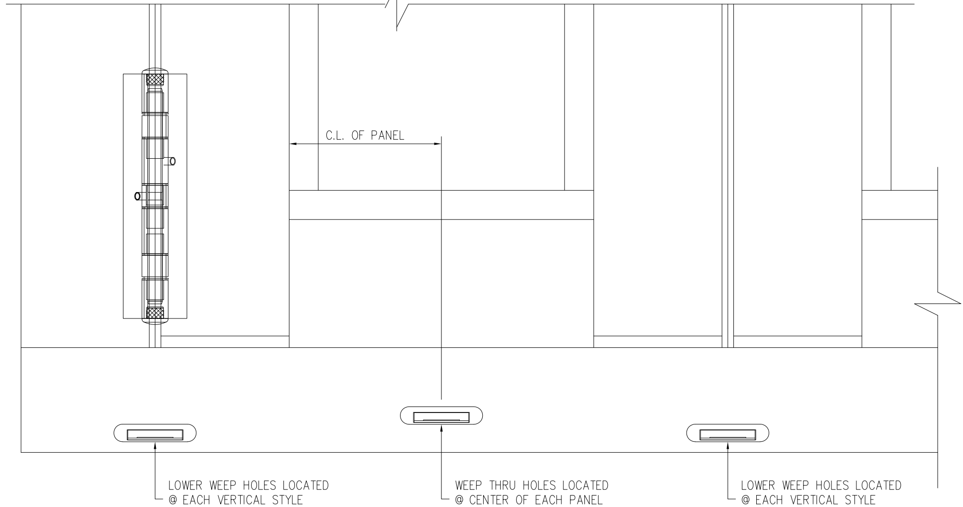
WEEP LOCATIONS
