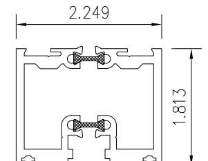
18 FRAME NARROW
