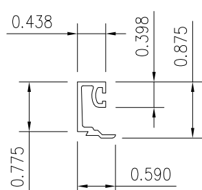
1/2" GLASS STOP
