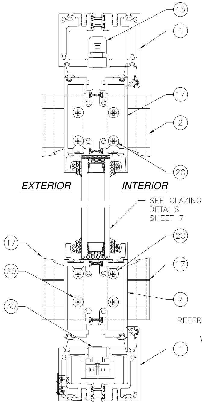
C 6 VERTICAL CROSS SECTION OUTFOLD BOTTOM LOAD
