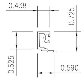
8 1" GLASS STOP
