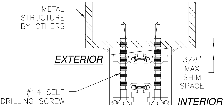
JAMB INSTALLATION DETAIL METAL STRUCTURE S47543 NO REINFORCEMENT
