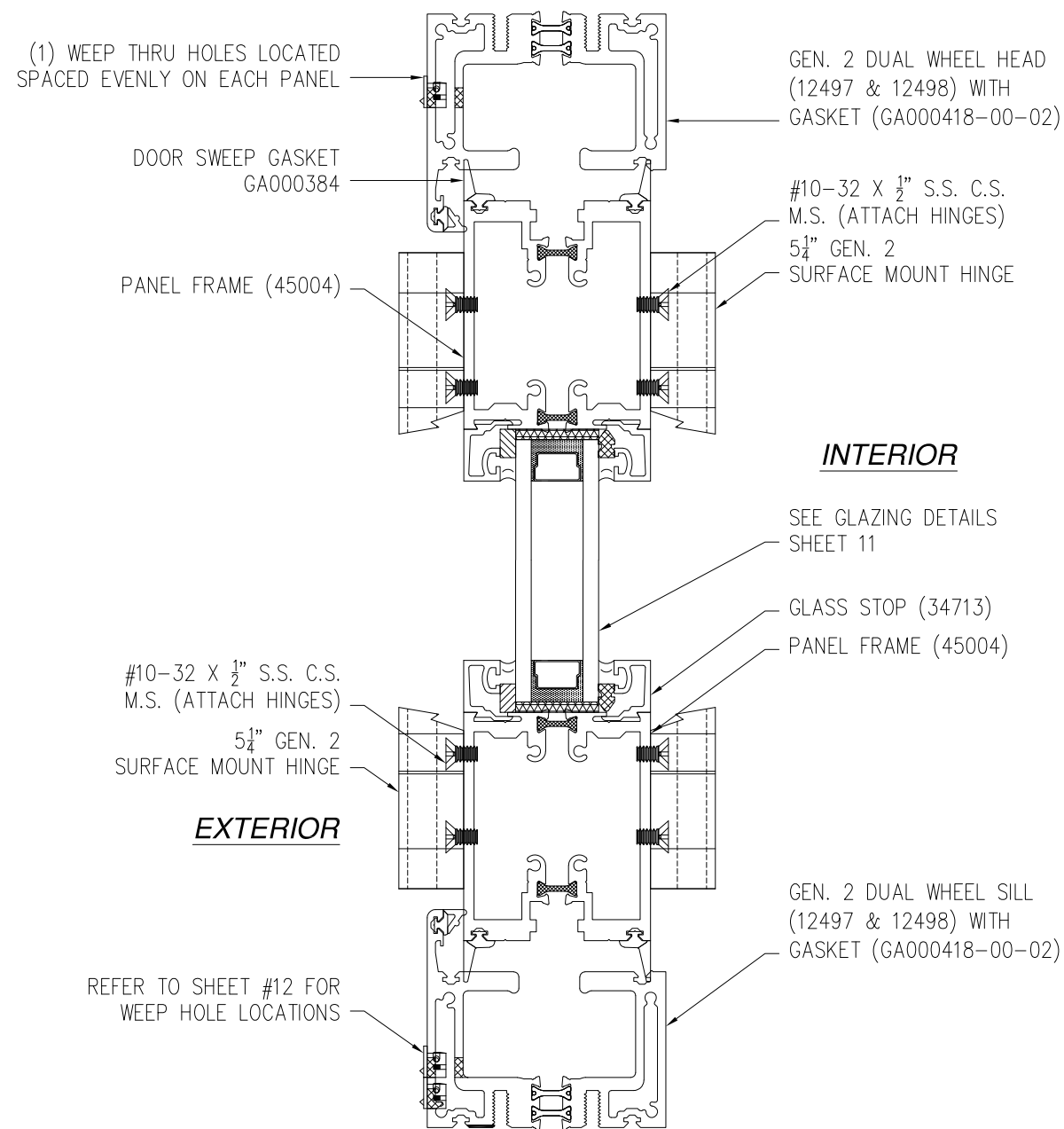
VERTICAL CROSS SECTION STANDARD WET GLAZED
