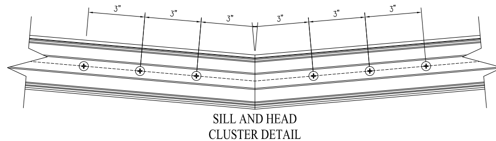
ANCHOR LAYOUT APPLIES TO ALL CONFIGURATIONS
