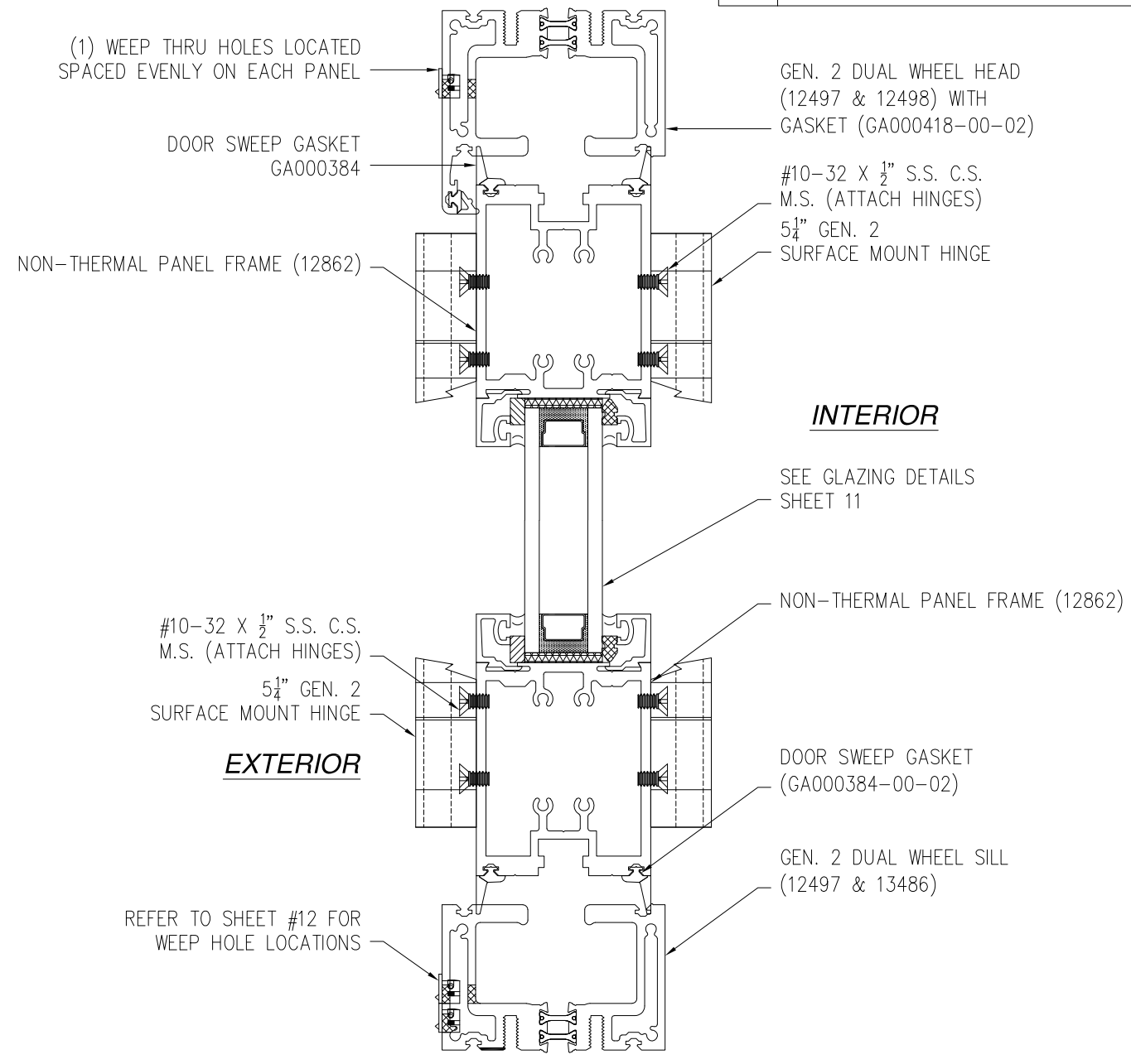
VERTICAL CROSS SECTION FLUSH SILL WET GLAZED
