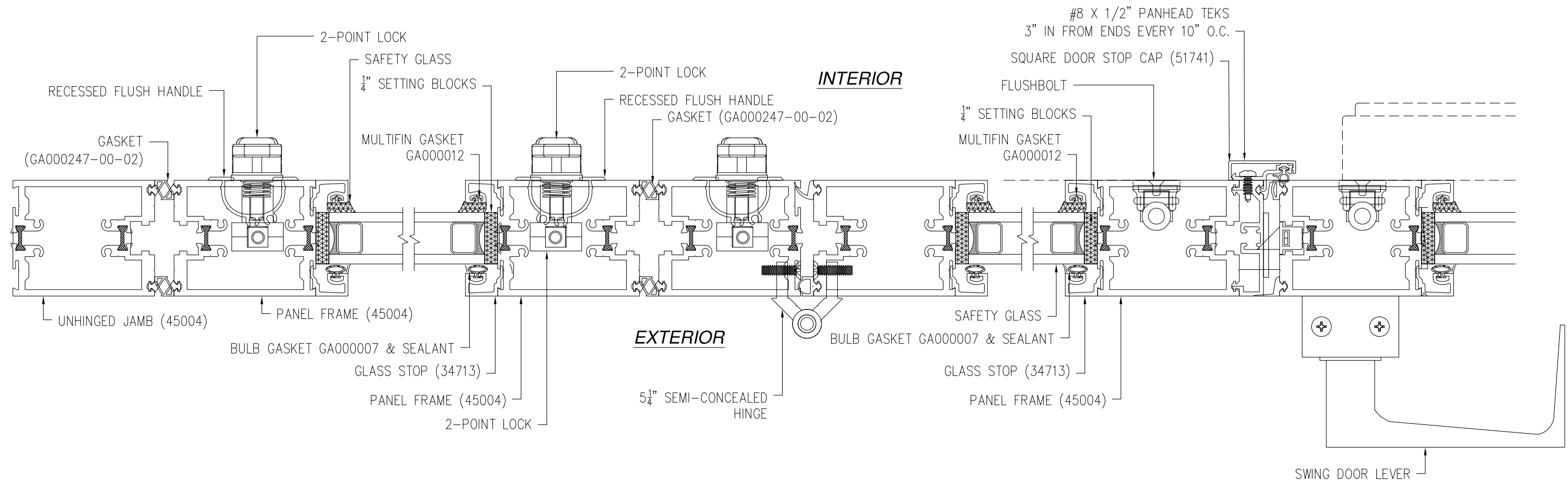
HORIZONTAL CROSS SECTION
