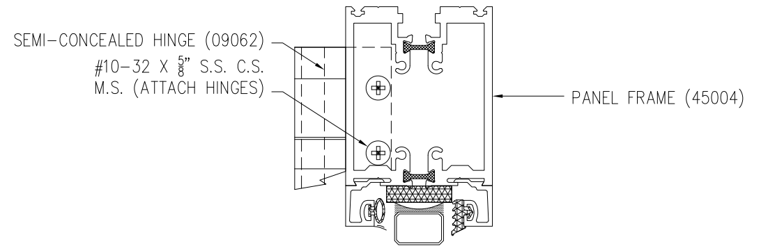
CONCEALED HINGE DETAIL
