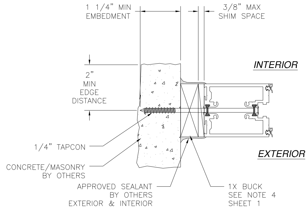
JAMB CROSS SECTION CONCRETE/MASONRY INSTALLATION
