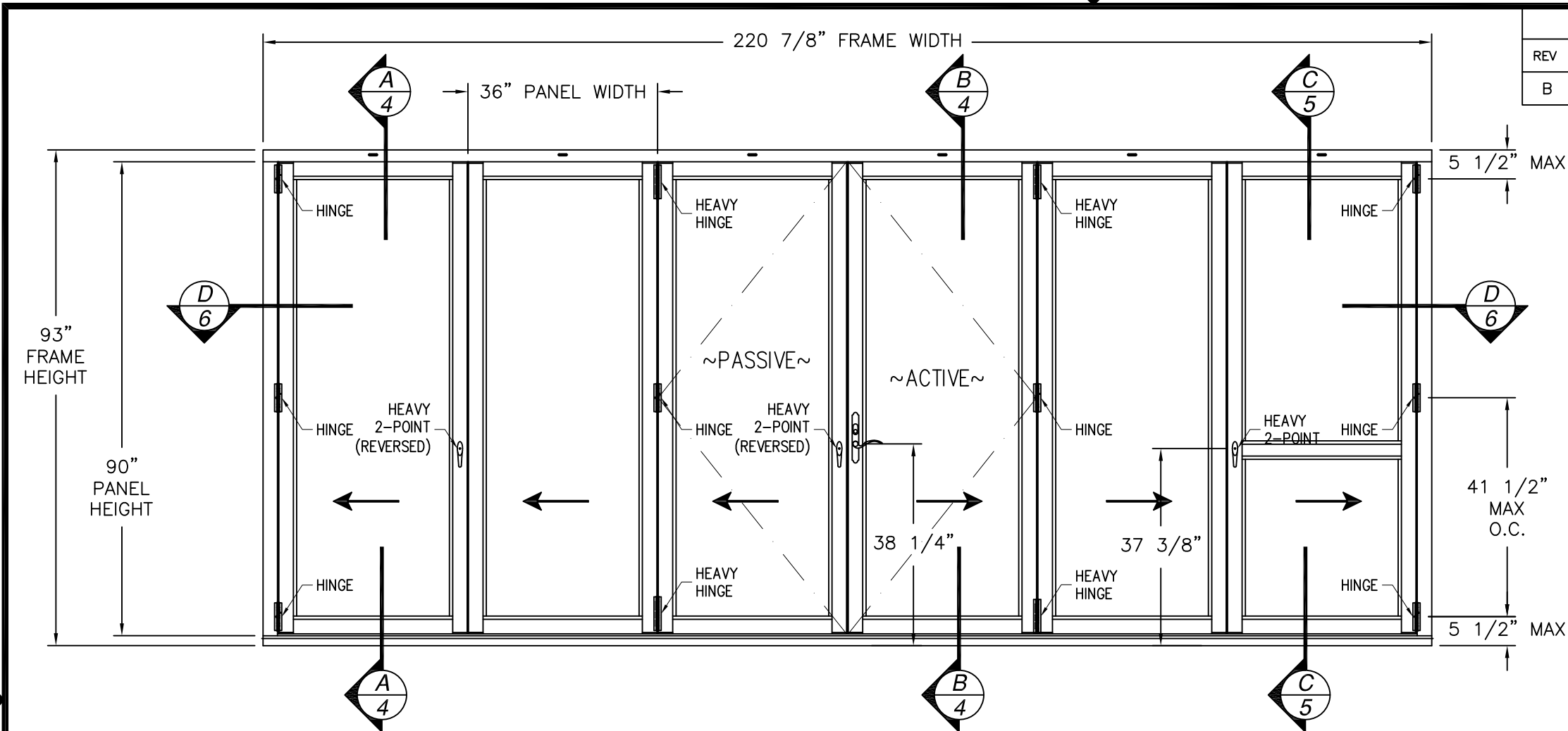
SERIES SI3000 IMPACT FGW 3' X 7.6' PANEL
