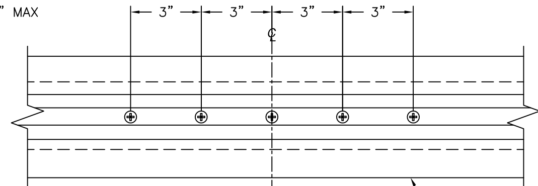
DETAIL F ANCHOR CLUSTER AT SILL
