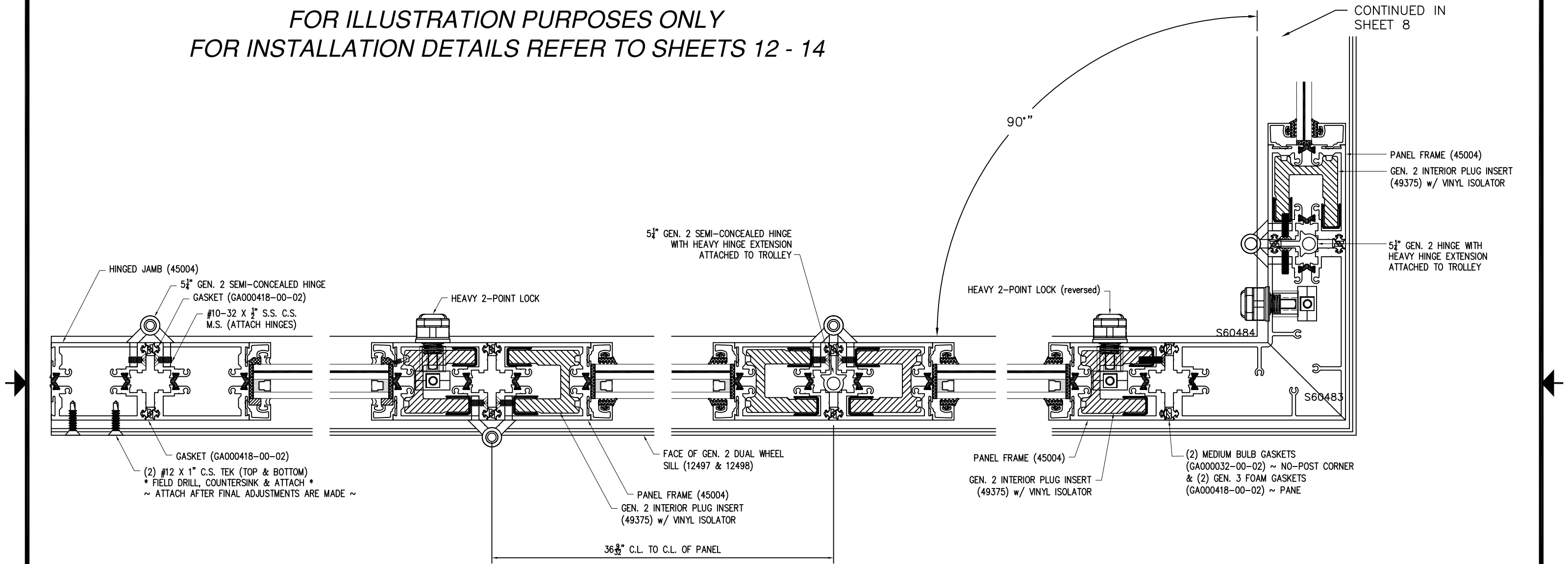
E 7 HORIZONTAL CROSS SECTION
