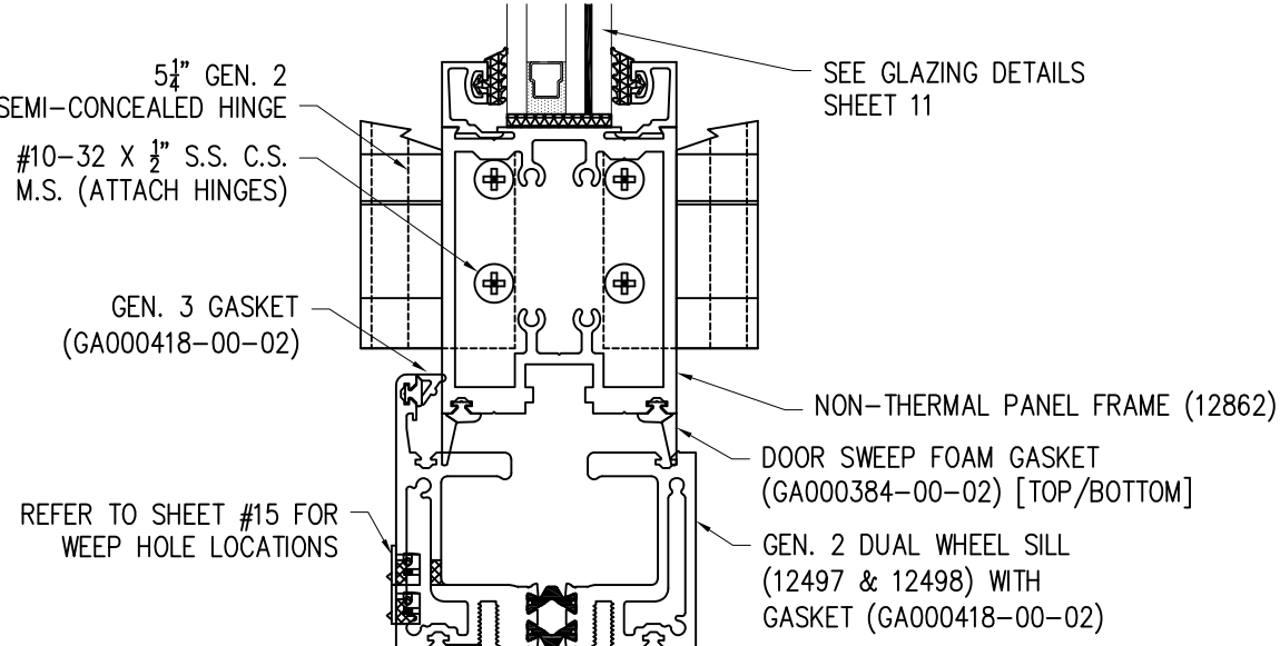
VERTICAL CROSS SECTION DRY GLAZED WITH NON-THERMAL PANEL
