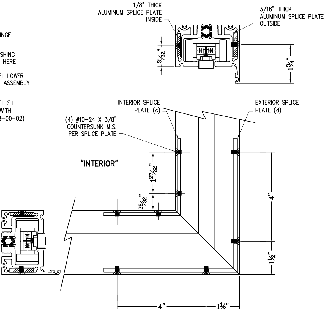
SPLICE PLATES INSTALLATION DETAIL
