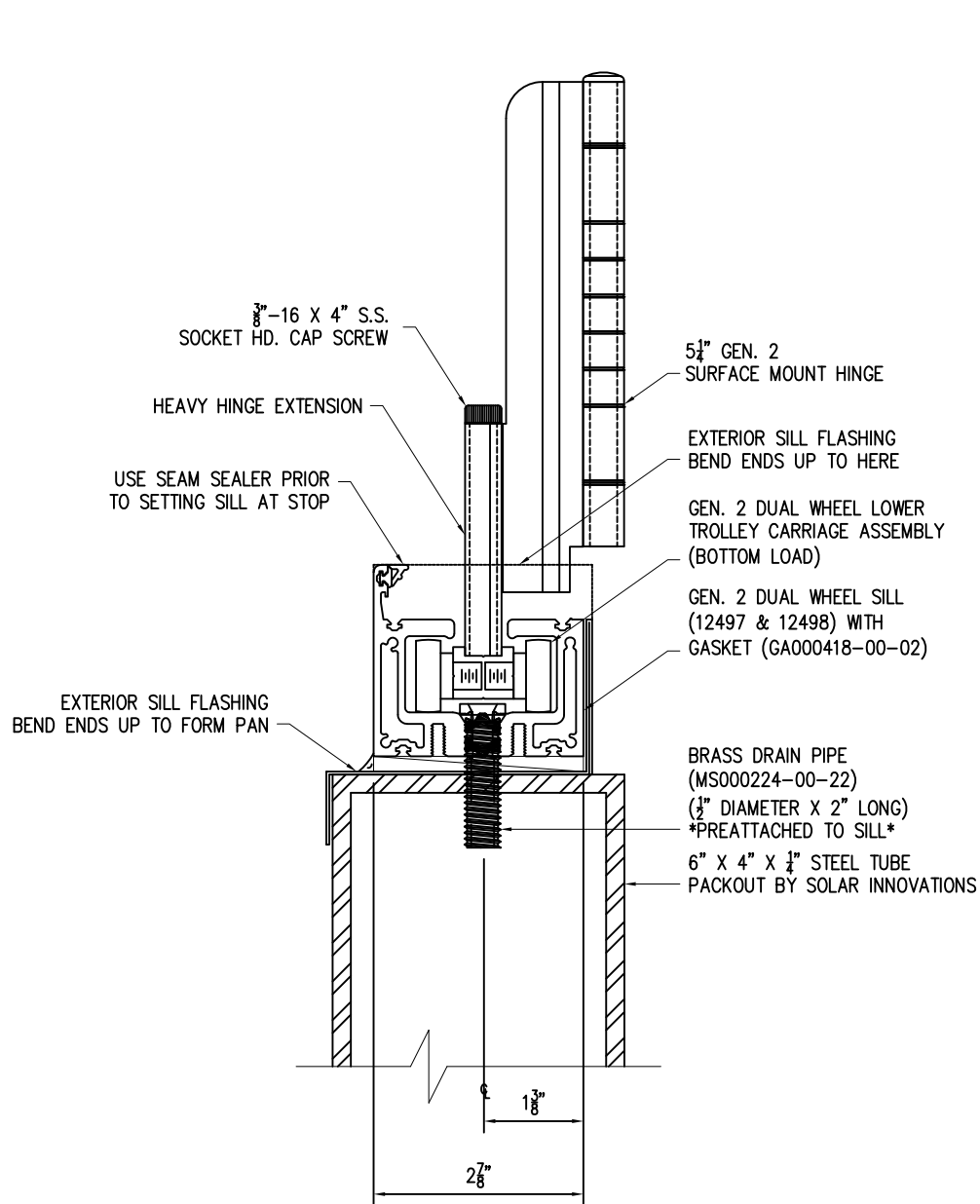
DRAIN PIPE AND HINGE EXTENSION DETAIL
