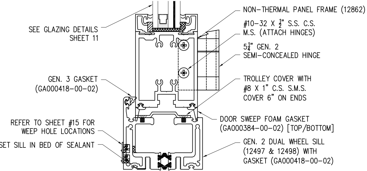
VERTICAL CROSS SECTION WET GLAZED WITH NON-THERMAL PANEL
