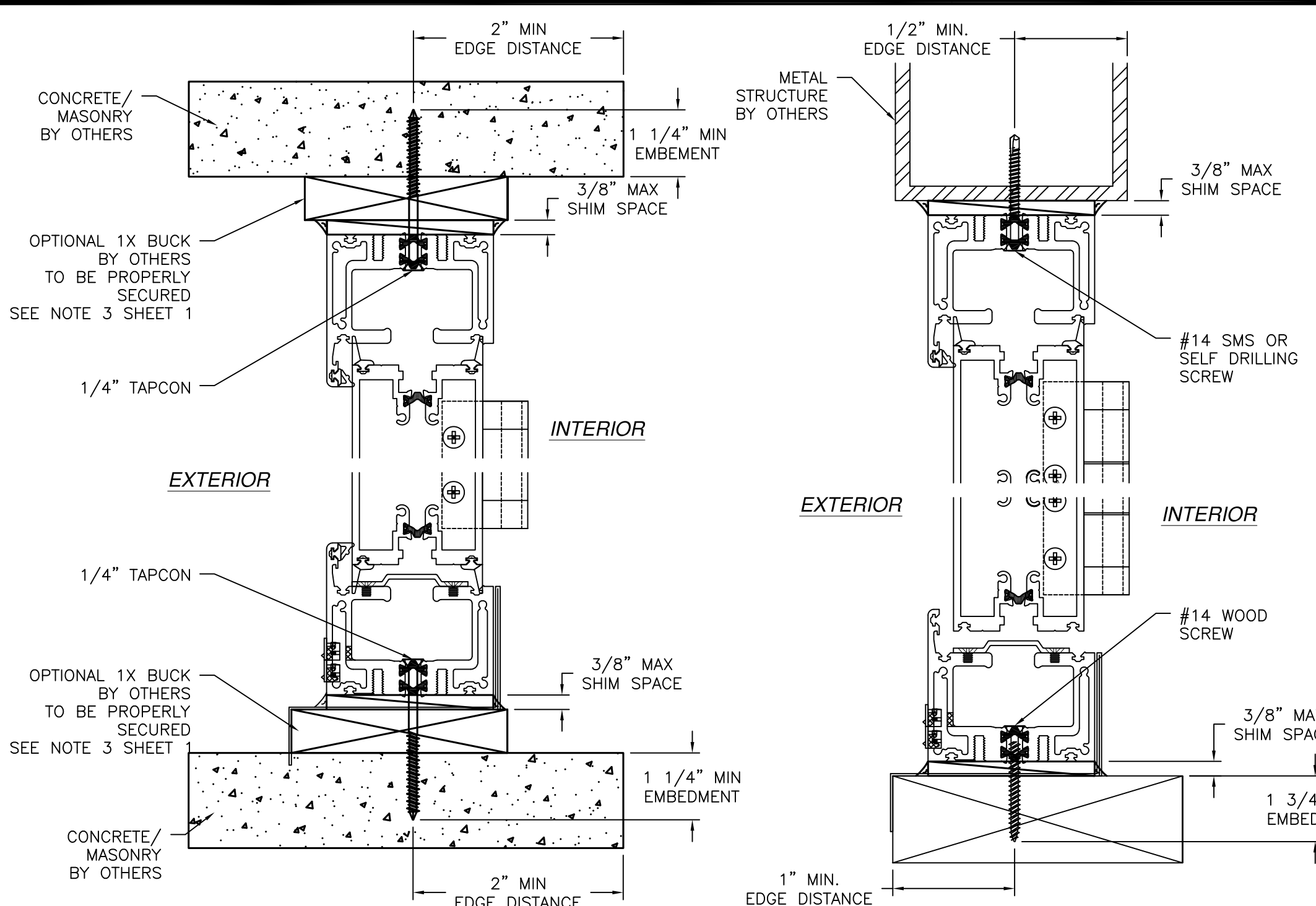
VERTICAL CROSS SECTION WOOD FRAMING OR 2X BUCK OR METAL STRUCTURE INSTALLATION STANDARD SILL SHOWN FLUSH SILL SIMILAR
