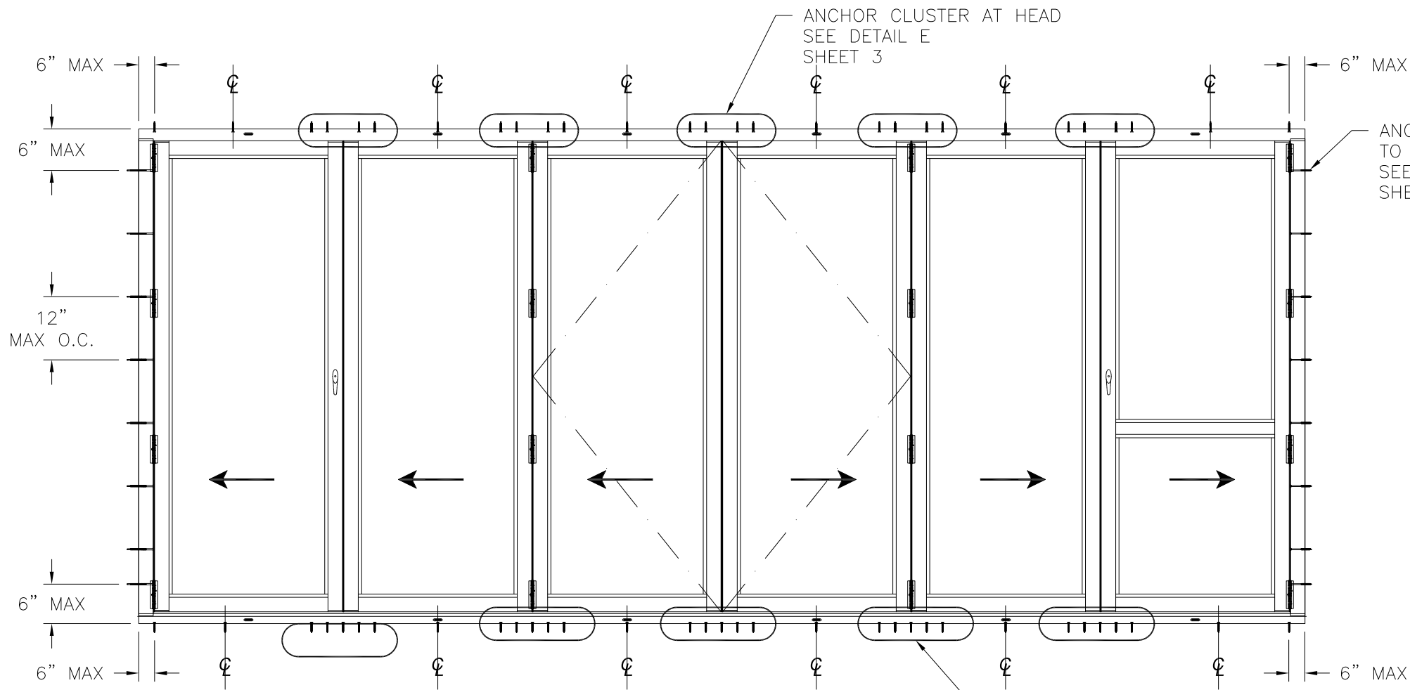
ANCHOR LAYOUT APPLICABLE TO ALL CONFIGURATIONS
