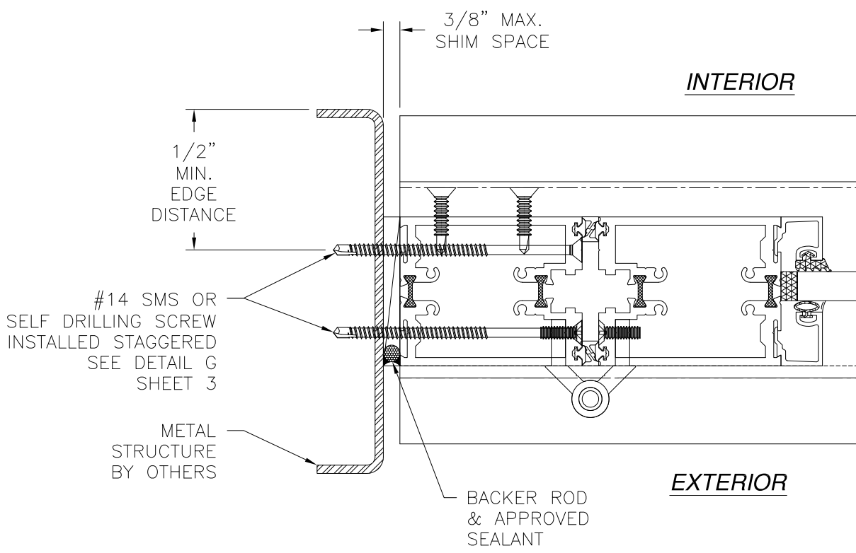
JAMB INSTALLATION DETAIL METAL STRUCTURE INSTALLATION
