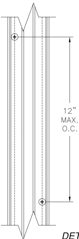
DETAIL G JAMB ANCHOR INSTALLATION
