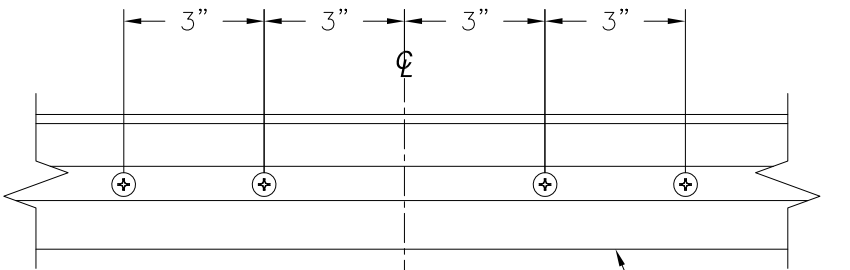
DETAIL E ANCHOR CLUSTER AT HEAD
