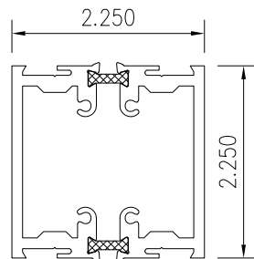
43 MULLION FRAME
