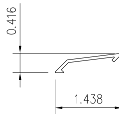
15 5 1/4" HINGE COVER
