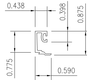
1/2" GLASS STOP
