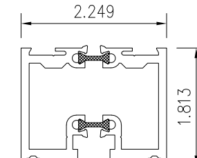
18 FRAME NARROW
