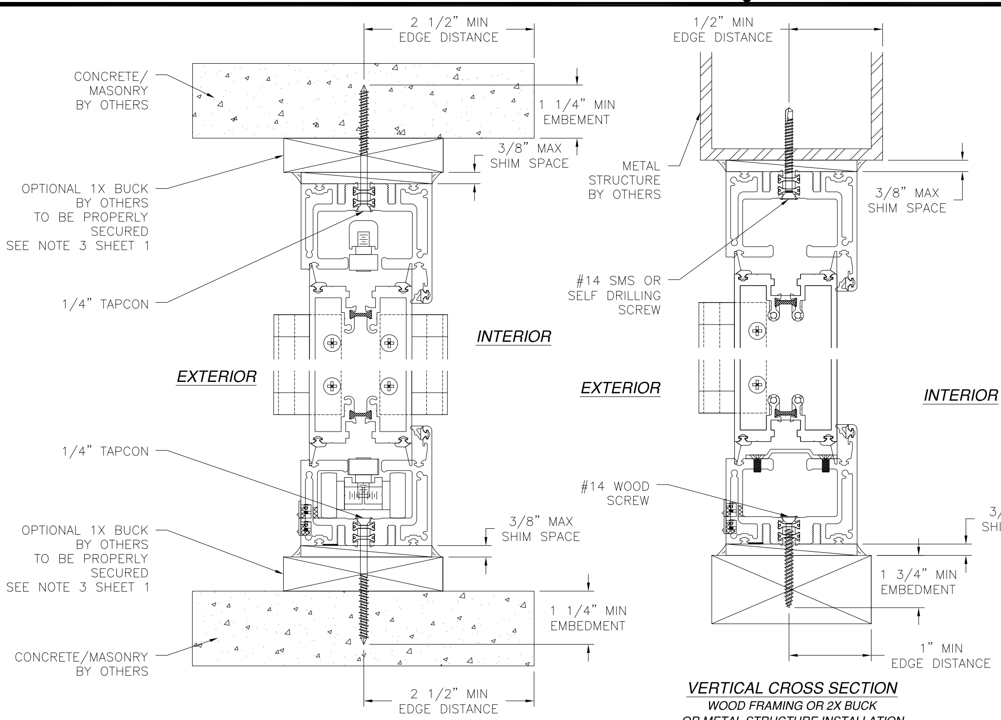
VERTICAL CROSS SECTION CONCRETE/MASONRY INSTALLATION STANDARD SILL SHOWN FLUSH SILL SIMILAR VERTICAL CROSS SECTION WOOD FRAMING OR 2X BUCK OR METAL STRUCTURE INSTALLATION STANDARD SILL SHOWN FLUSH SILL SIMILAR
