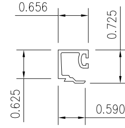
9 9/16" GLASS STOP
