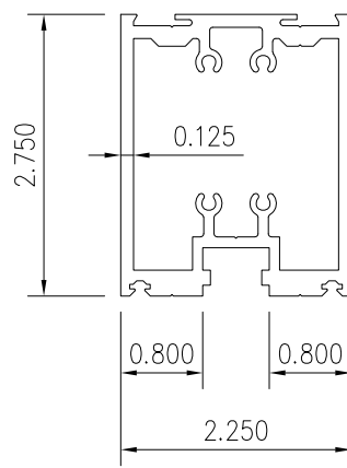
49 REGULAR NON-THERMAL FRAME
