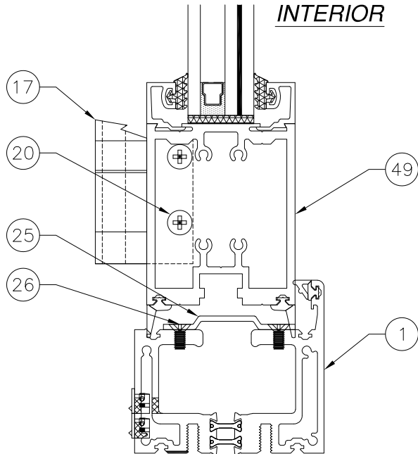
A 7 VERTICAL CROSS SECTION NON-THERMAL PANEL
