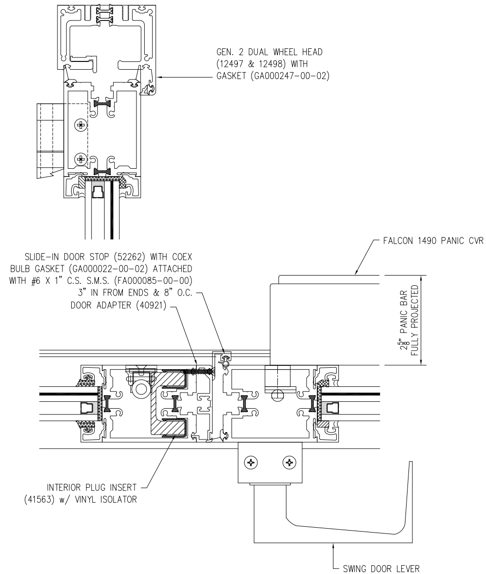
PANIC BAR DETAILS
