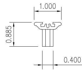
6 LOW-PROFILE HANDLE
