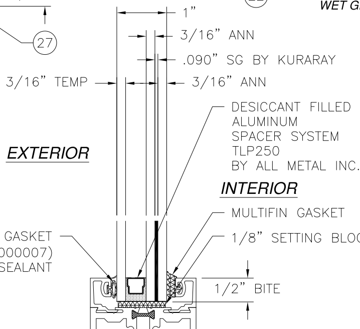
GLAZING G BULB GASKET & MULTIFIN GLAZING
