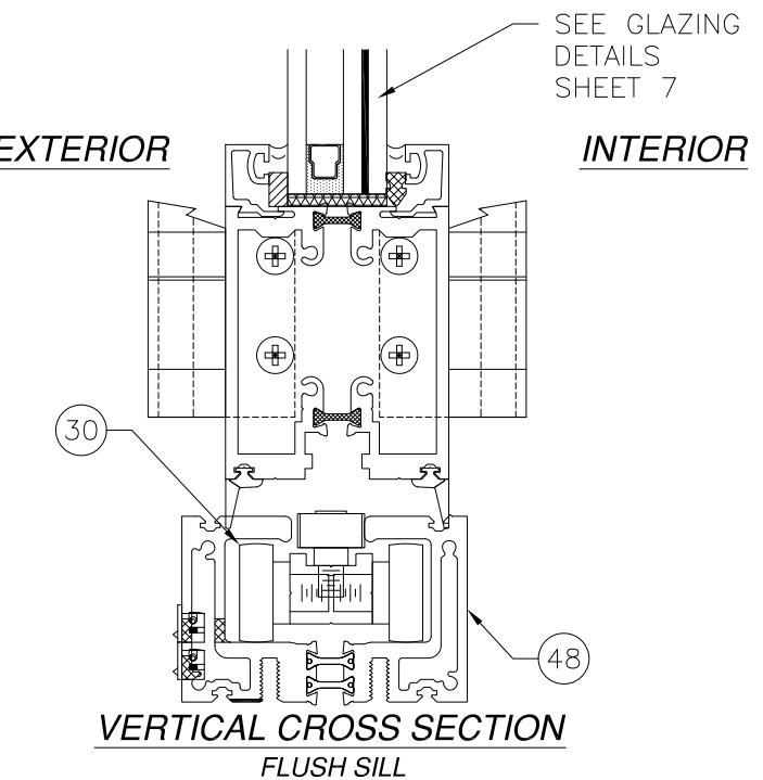
H 6 VERTICAL CROSS SECTION FLUSH SILL
