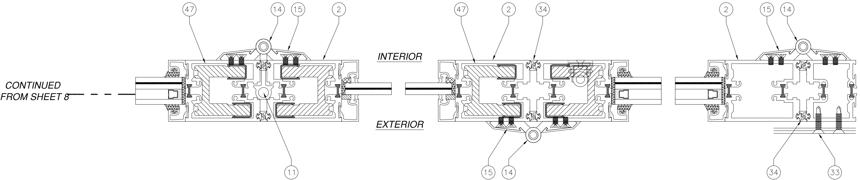
D 9 HORIZONTAL CROSS SECTION
