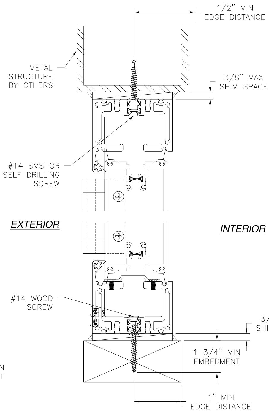
VERTICAL CROSS SECTION WOOD FRAMING OR 2X BUCK OR METAL STRUCTURE INSTALLATION STANDARD SILL, FLUSH SILL SIMILAR
