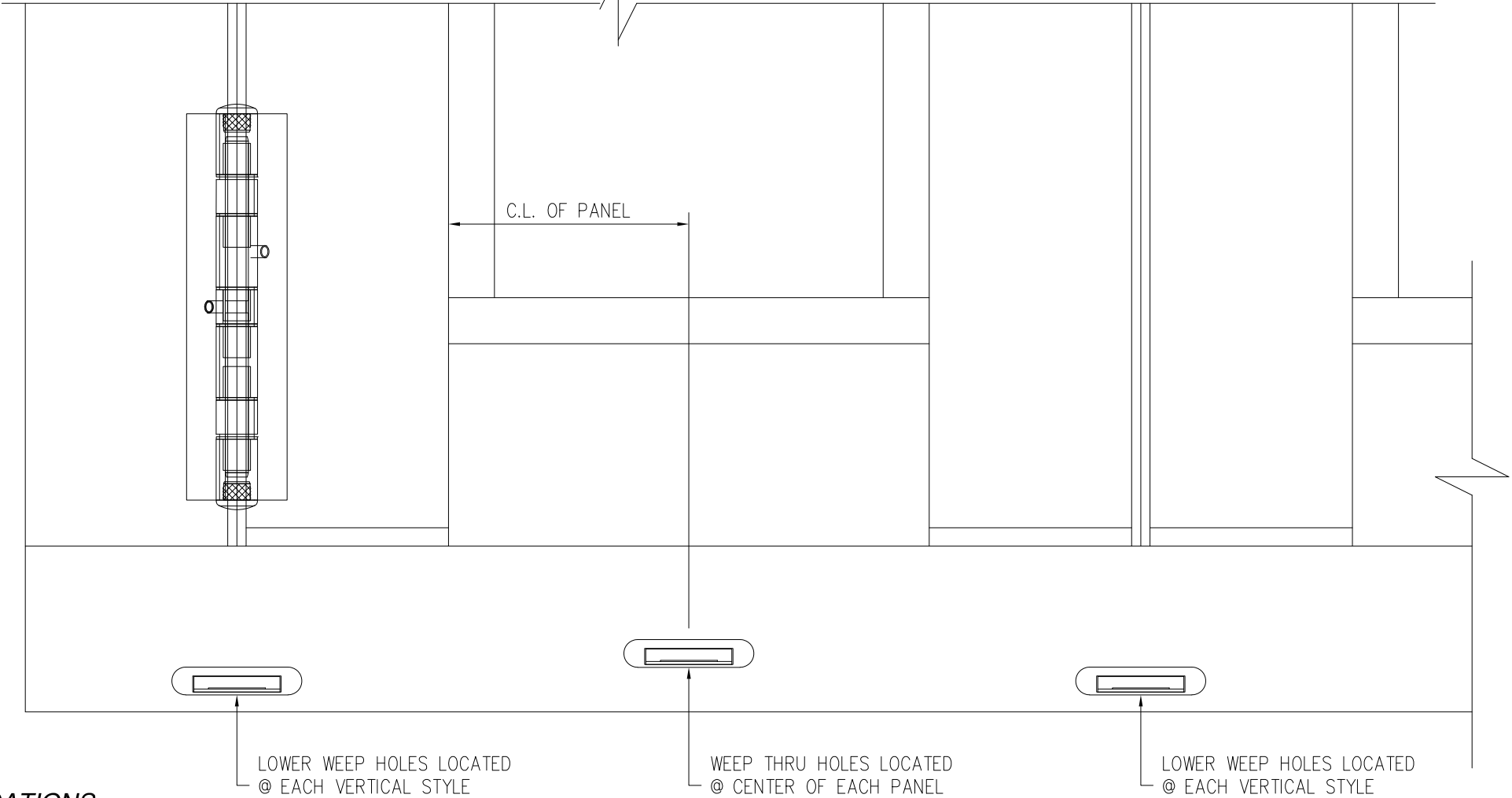
WEEP LOCATIONS
