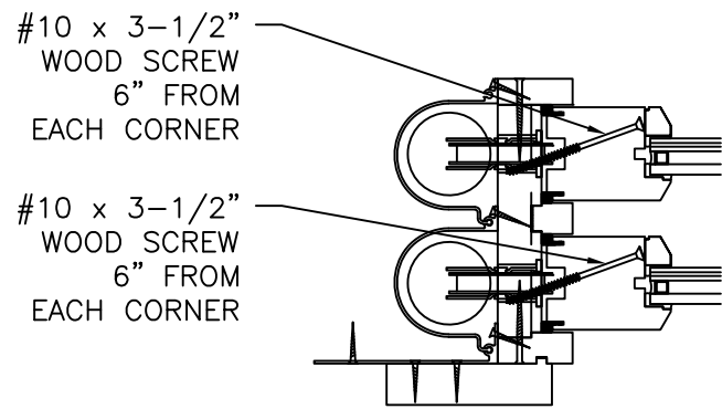
FIXED WINDOW HORIZONTAL CROSS SECTION LEFT SIDE SHOWN RIGHT SIDE SIMILAR
