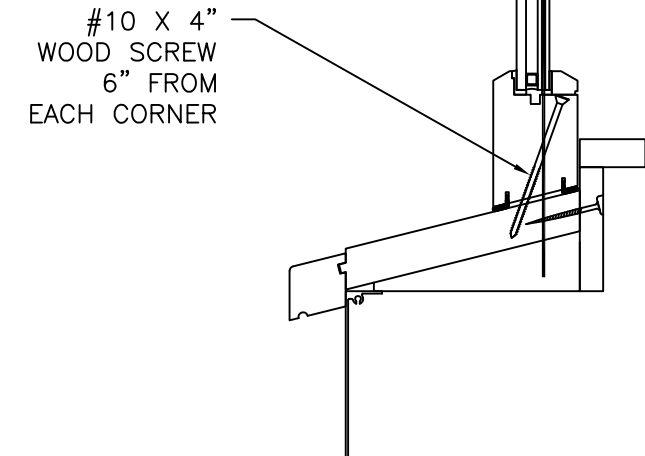
FIXED WINDOW VERTICAL CROSS SECTION
