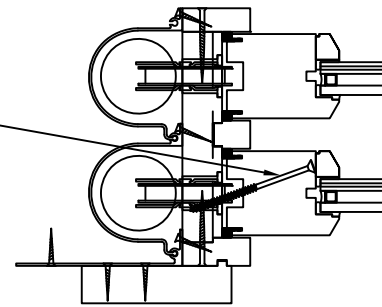
SINGLE HUNG WINDOW HORIZONTAL CROSS SECTION LEFT SIDE SHOWN RIGHT SIDE SIMILAR
