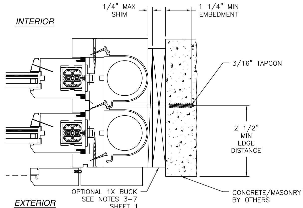
JAMB INSTALLATION DETAIL CONCRETE/MASONRY FRAMING
