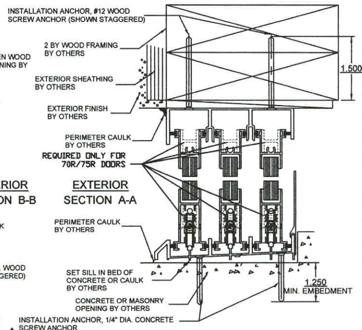
TYPICAL DETAIL AT 2 BY WOOD FRAMING
