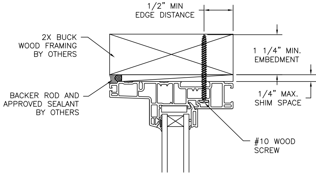
EXTERIOR INTERIOR
