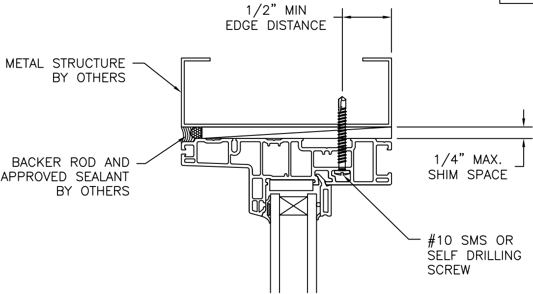
EXTERIOR INTERIOR
