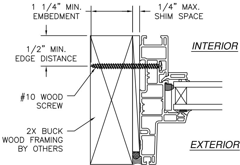
HORIZONTAL CROSS SECTION 2X BUCK/WOOD FRAMING INSTALLATION
