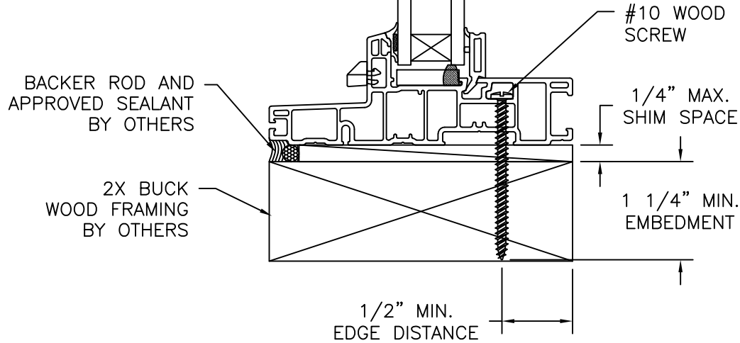
VERTICAL CROSS SECTION 2X BUCK/WOOD FRAMING INSTALLATION
