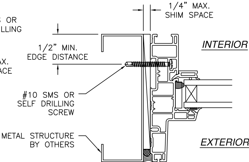
HORIZONTAL CROSS SECTION METAL STRUCTURE INSTALLATION
