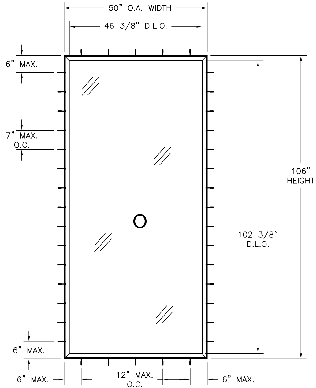
S-4200 PRESTIGE PVC FIXED WINDOW EXTERIOR VIEW
