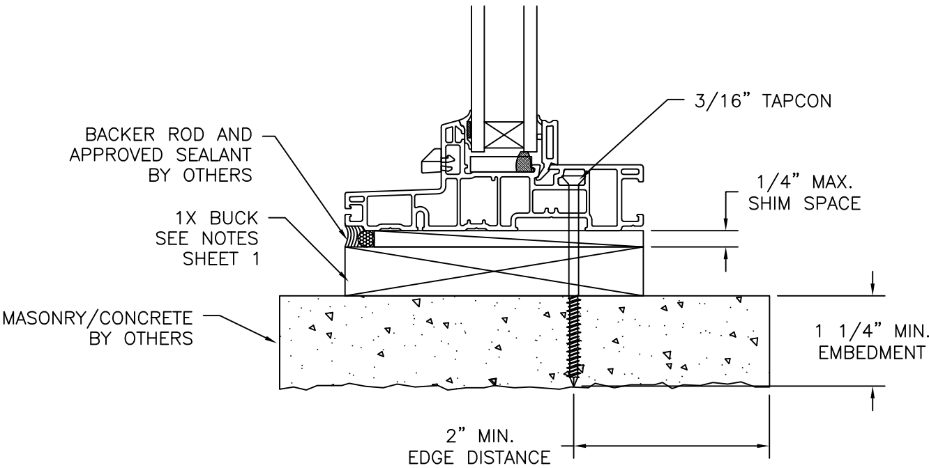
VERTICAL CROSS SECTION MASONRY/CONCRETE INSTALLATION
