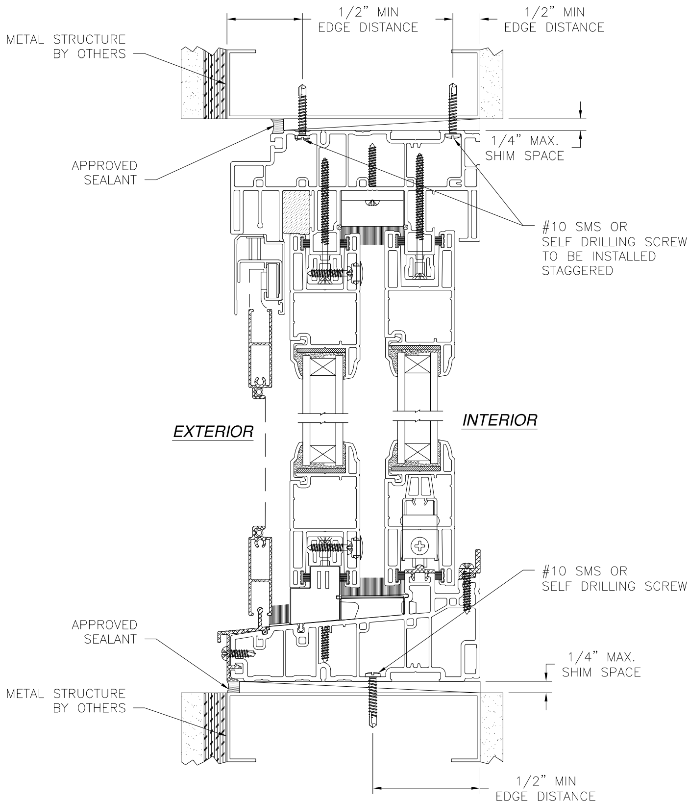
VERTICAL CROSS SECTION METAL STRUCTURE INSTALLATION
