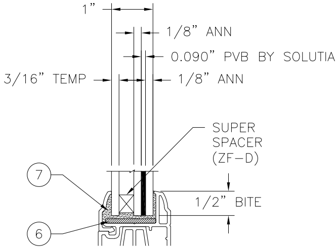
GLAZING DETAIL
