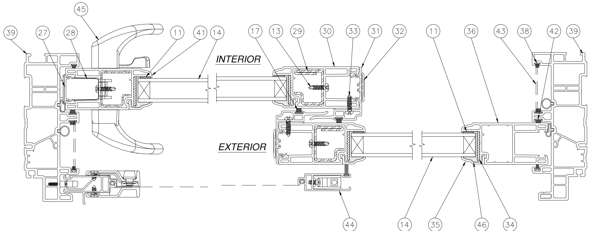
HORIZONTAL CROSS SECTION
