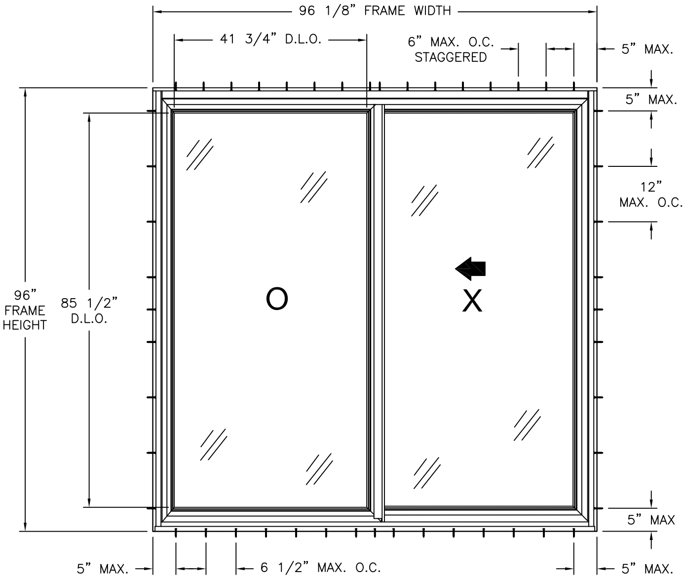
REINFORCED VINYL SLIDING GLASS DOOR EXTERIOR VIEW
