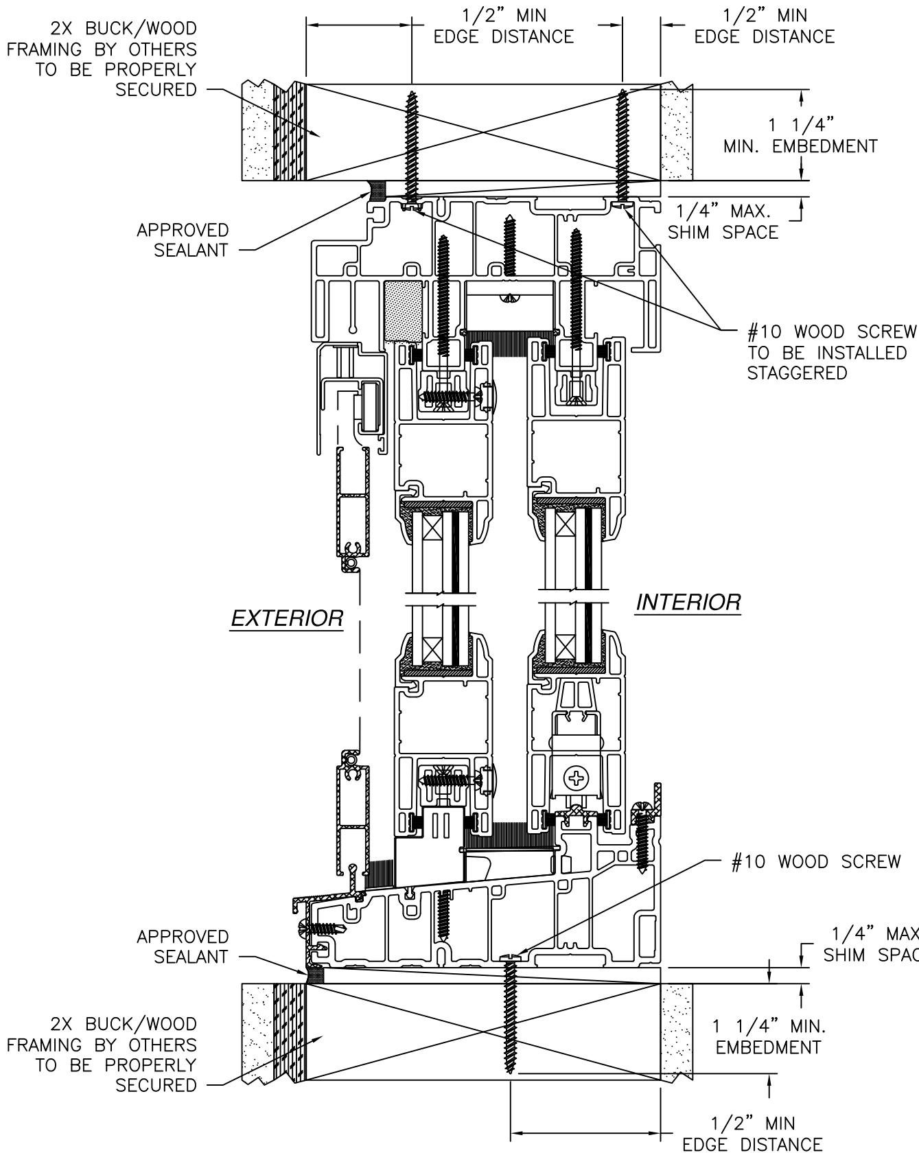
VERTICAL CROSS SECTION 2X BUCK/WOOD FRAMING INSTALLATION
