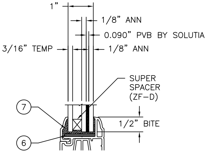
GLAZING DETAIL
