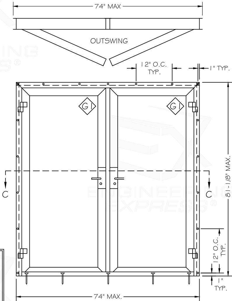
A OUTSWING ELEVATION
