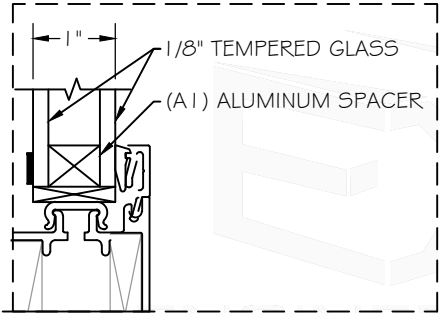
(G1) GLASS DETAIL (NON IMPACT)
