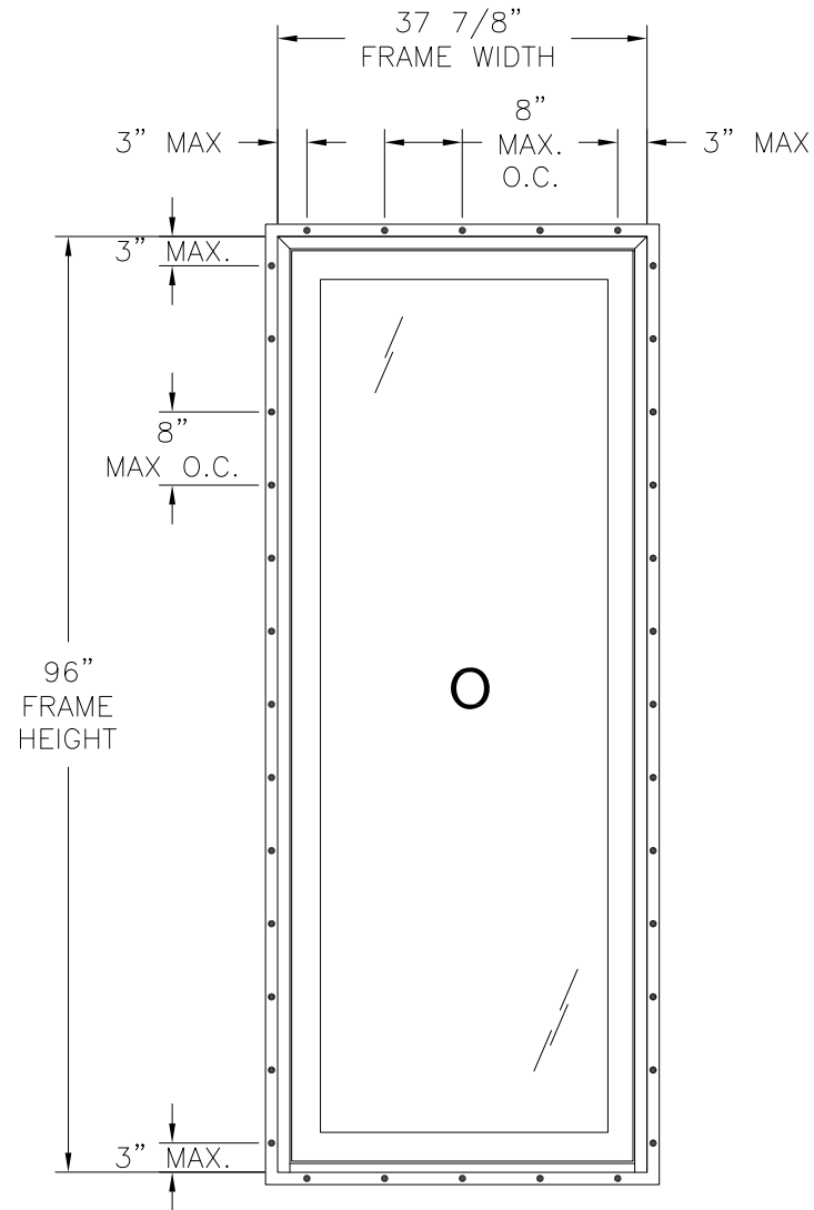
SERIES 9800 VINYL FIXED SIDELITE FIN INSTALLATION
