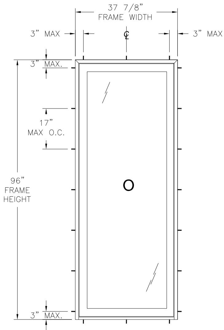
SERIES 9800 VINYL FIXED SIDELITE EXTERIOR VIEW FRAME INSTALLATION
