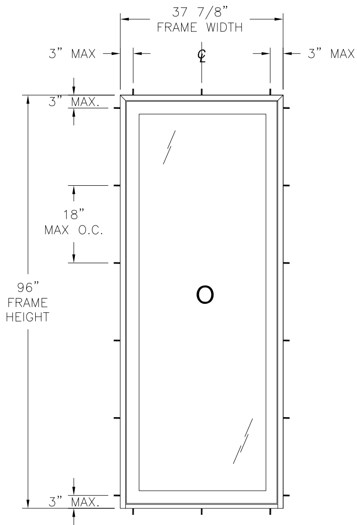
SERIES 9800 VINYL FIXED SIDELITE EXTERIOR VIEW STEEL STRAP INSTALLATION
