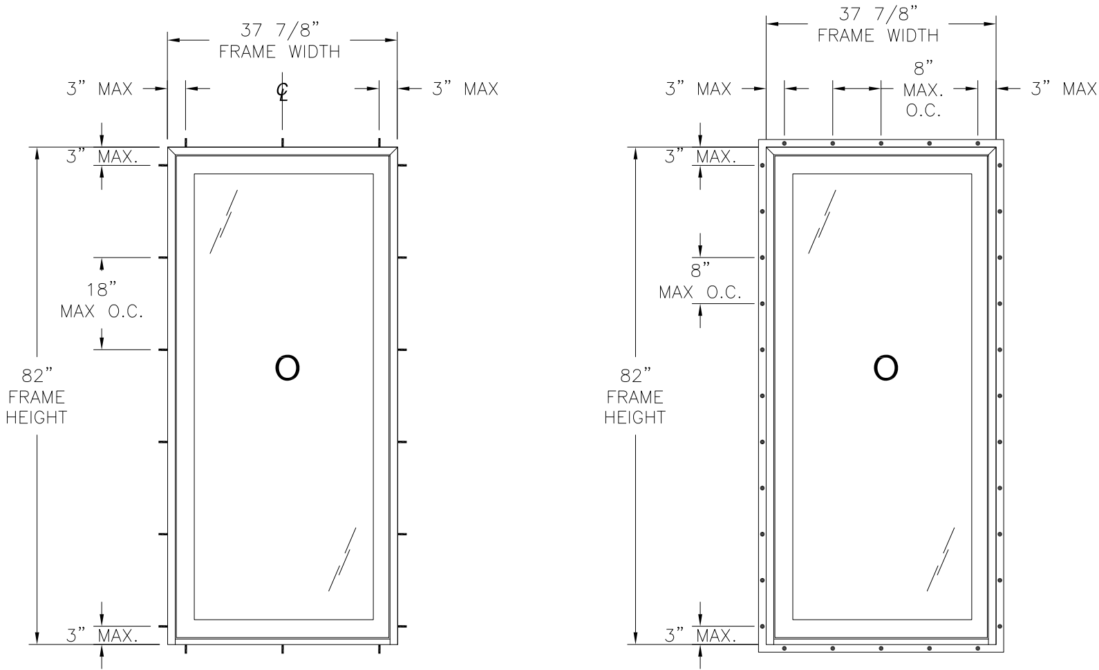
SERIES 9800 VINYL FIXED SIDELITE EXTERIOR VIEW FRAME AND STEEL STRAP INSTALLATION
