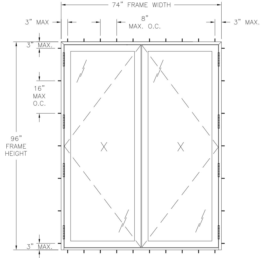
SERIES 9800 VINYL HINGED PATIO DOOR EXTERIOR VIEW FRAME INSTALLATION THROUGH THE FRAME
