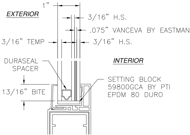
GLAZING DETAIL
