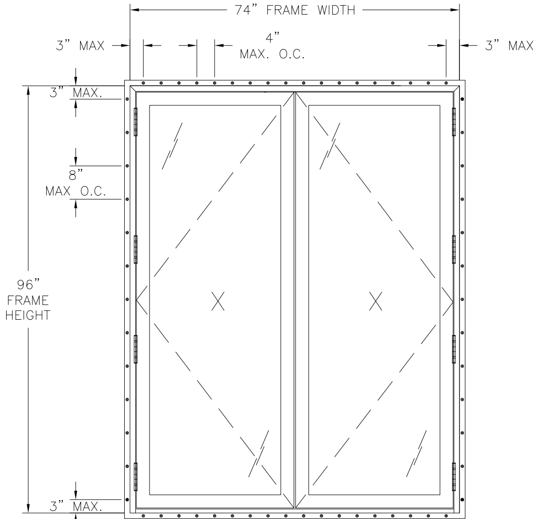
SERIES 9800 VINYL HINGED PATIO DOOR EXTERIOR VIEW FIN INSTALLATION WITH ROOFING NAILS
