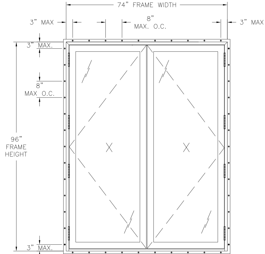
SERIES 9800 VINYL HINGED PATIO DOOR EXTERIOR VIEW FIN INSTALLATION WITH WOOD SCREWS
