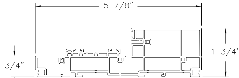
MAIN FRAME VINYL PVC (VM1220)
