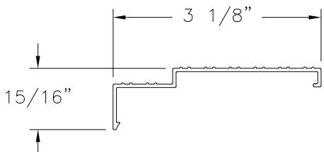
SILL RISER ALUMINUM 6063-T5
