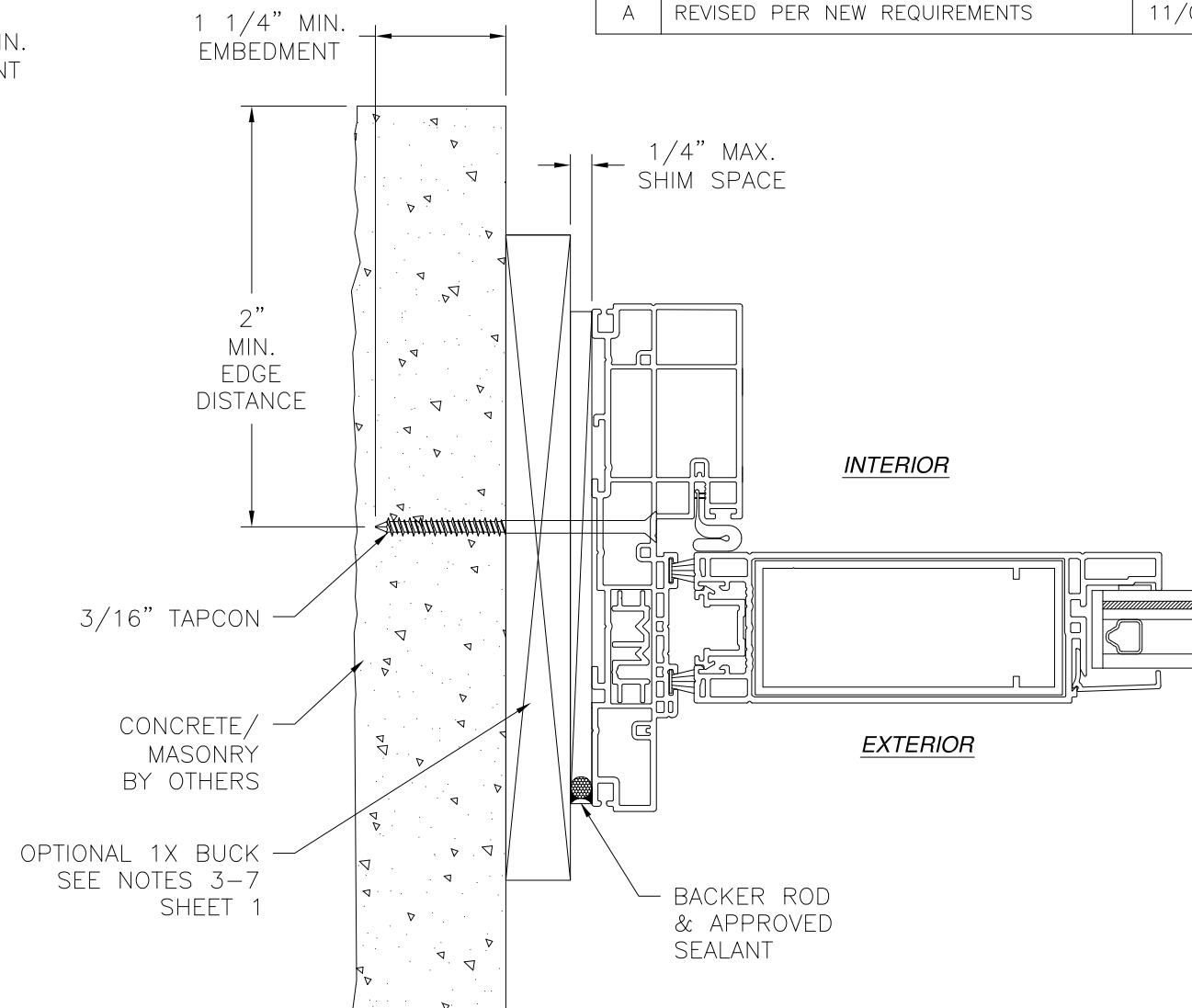
JAMB INSTALLATION DETAIL CONCRETE/MASONRY INSTALLATION
