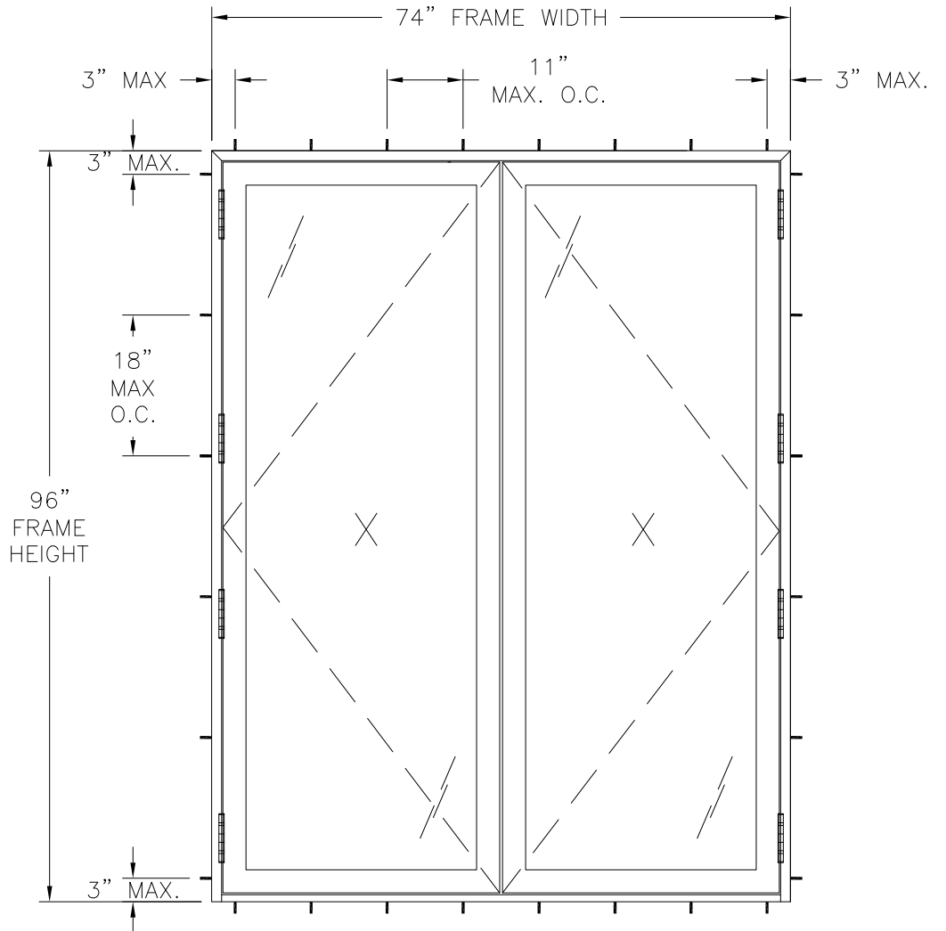
SERIES 9800 VINYL HINGED PATIO DOOR EXTERIOR VIEW FRAME INSTALLATION WITH STEEL STRAP
