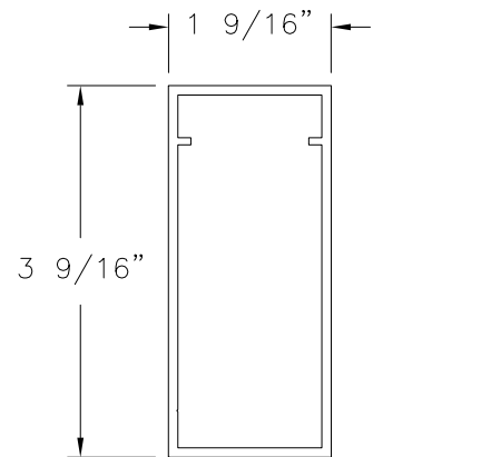
PANEL REINFORCEMENT ALUMINUM 6063-T5
