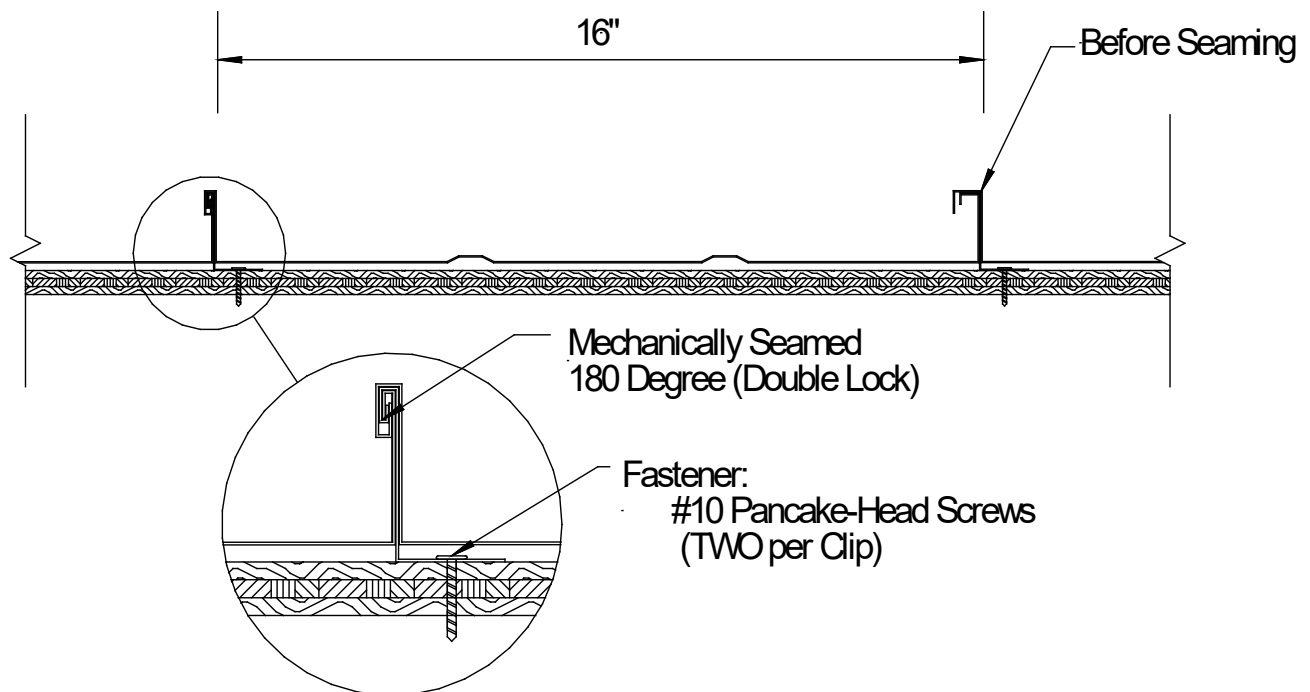
Typical Assembly Profile View (Typical Fastening Pattern Across Width)
