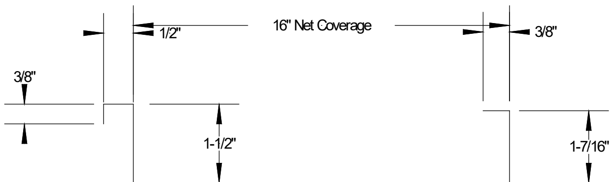
Panel Profile
