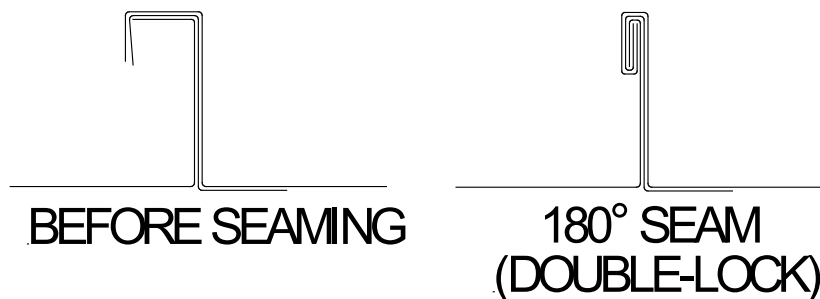
Typical Panel Seam
