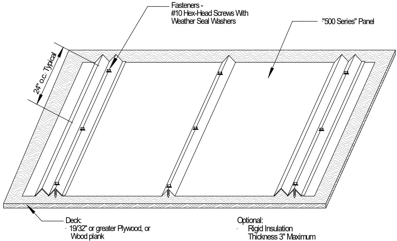
Typical Roof Assembly Isometric View
