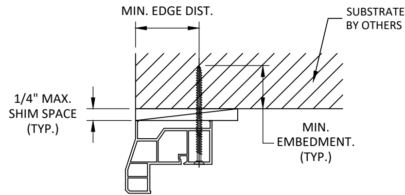
A 4 ANCHOR DETAIL THROUGH FRAME
