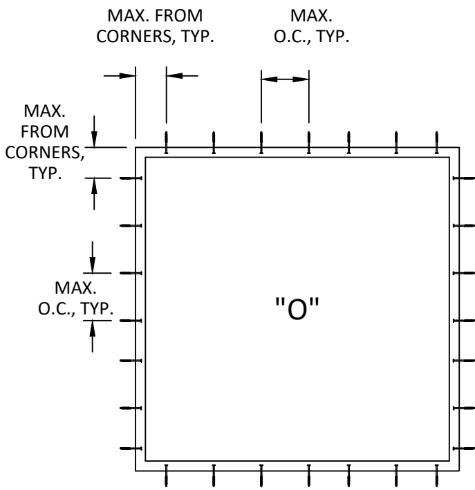
ANCHOR LAYOUT
