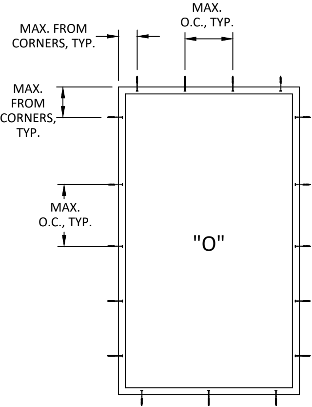
ANCHOR LAYOUT
