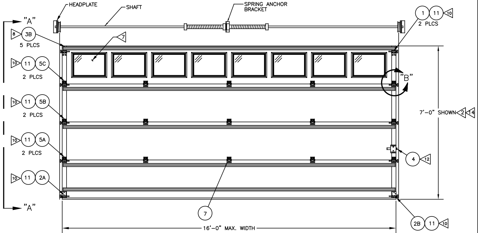
INTERIOR ELEVATION SCALE: 1/16"=1"
