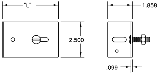
8 405964 & 046450, BRACKET, JAMB ATTACH TO TRACK WITH 1/4\"/>
