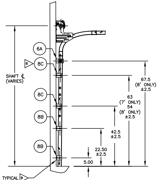
STANDARD TRACK DETAIL SCALE: 1/16" = 1"
