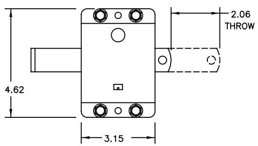
4 409334-0001 SLIDE LOCK ASSY ATTACH TO DOOR WITH 4 SCREWS P/N 605911-0001
