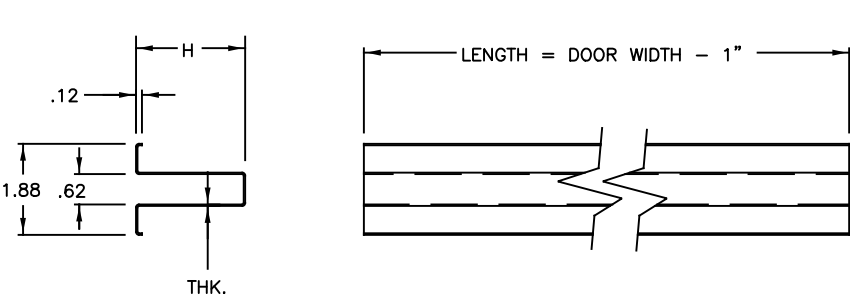
3 400650-XXX1, ROLLED HS STRUT
