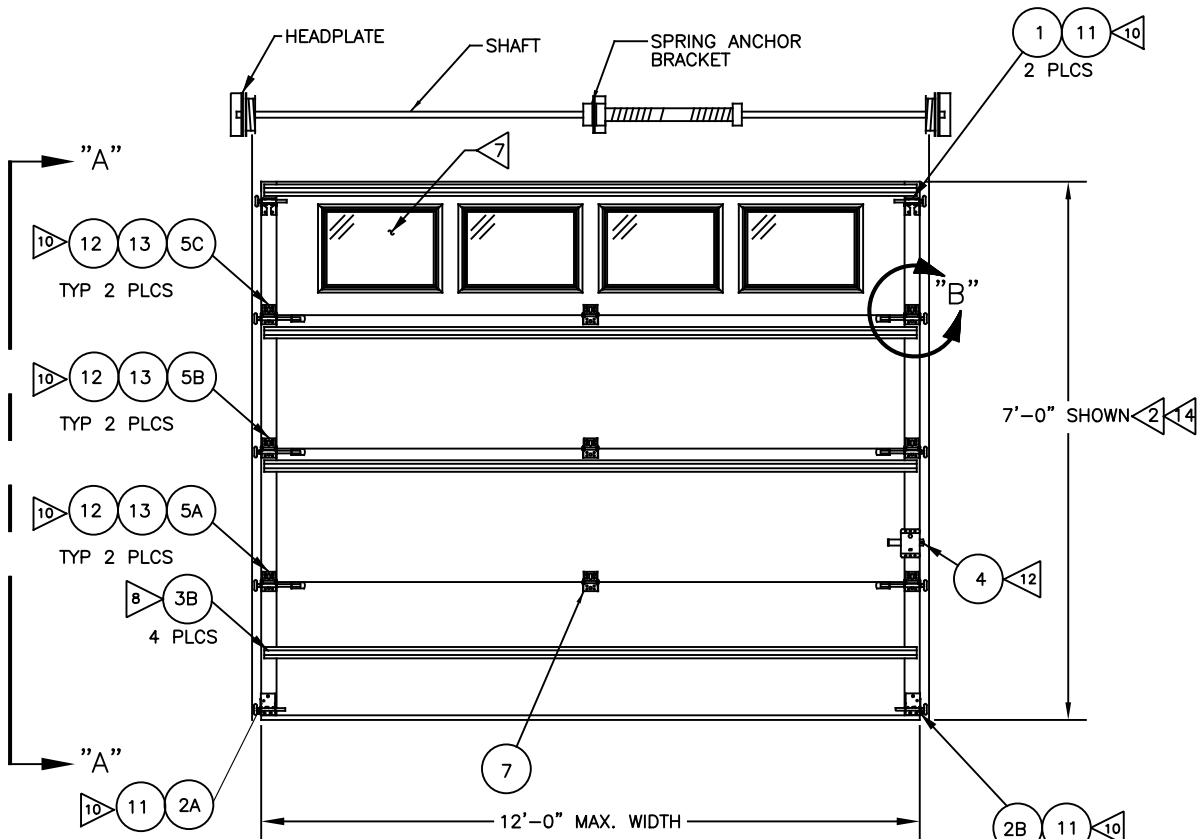
INTERIOR ELEVATION SCALE: 1/16"=1"
