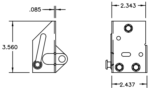
2 405771-XXXX BOT. FIXTURE ATTACH TO DOOR WITH 3 SCREWS P/N 605911-0001
