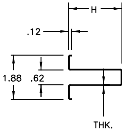
3 400650-XXX1, ROLLED HS STRUT
