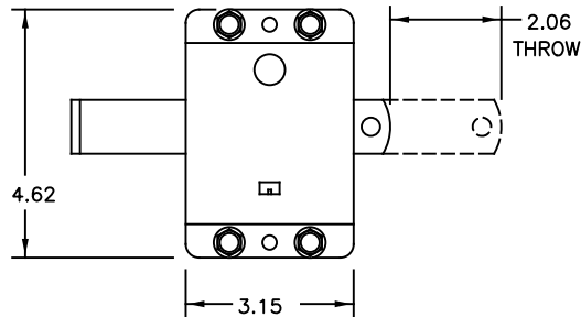
4 409334-0001 SLIDE LOCK ASSY ATTACH TO DOOR WITH 4 SCREWS P/N 605911-0001
