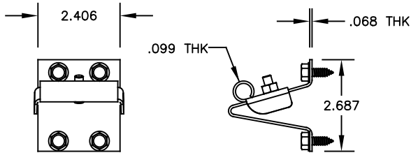
1 409808-0001, TOP FIXTURE ATTACH TO DOOR WITH 4 SCREWS P/N 605911-0001
