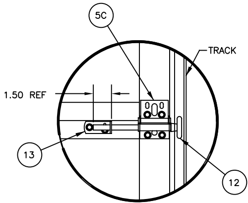
DETAIL "B" SCALE: 1/4
