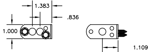
13 405742-0001, BRACKET, ROLLER SHAFT ATTACH TO DOOR WITH 2 SCREWS P/N 605911-0001 0.085" THK
