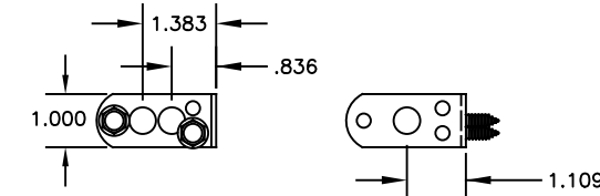
13 405742-0001, BRACKET, ROLLER SHAFT ATTACH TO DOOR WITH 2 SCREWS P/N 605911-0001 0.085\"/>
