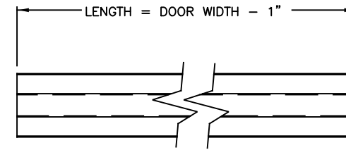
3 400650-XXX1, ROLLED HS STRUT
