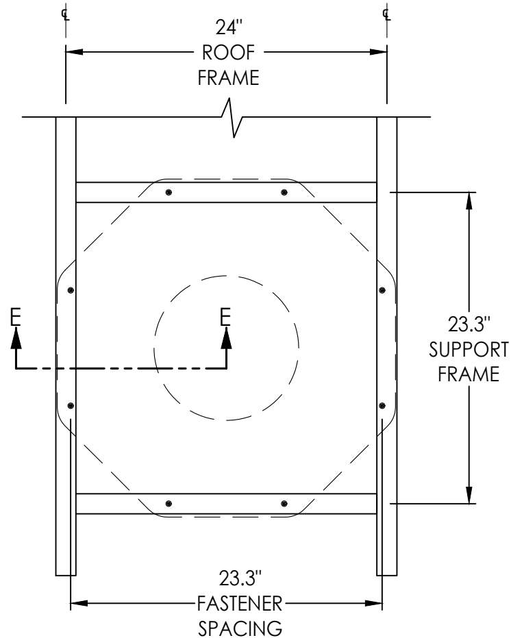
FRAMING DETAIL 14"
