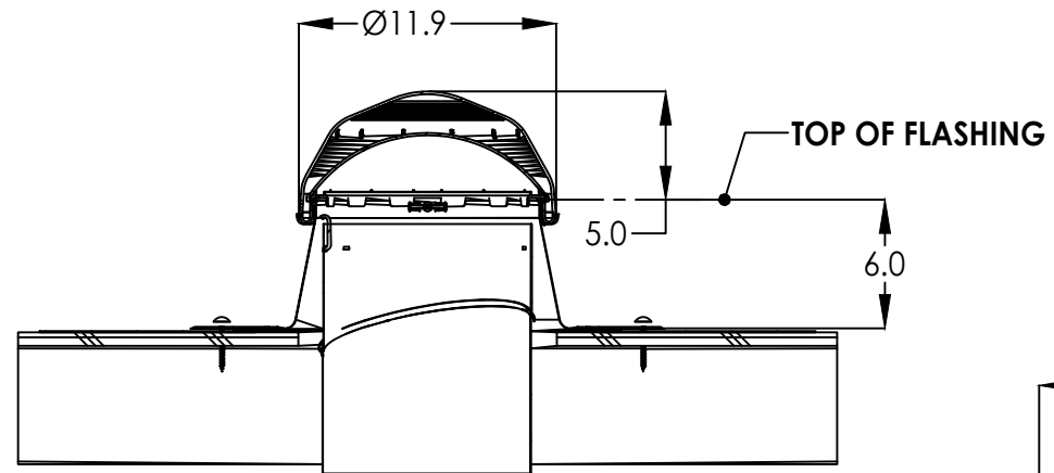
FLAT 6"
