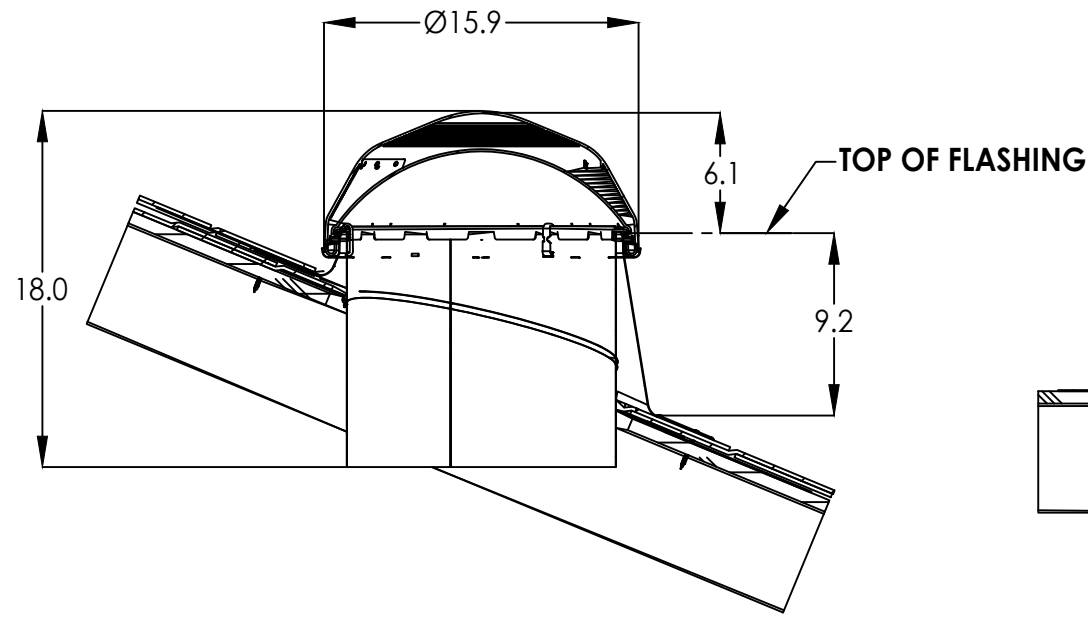
PITCHED
