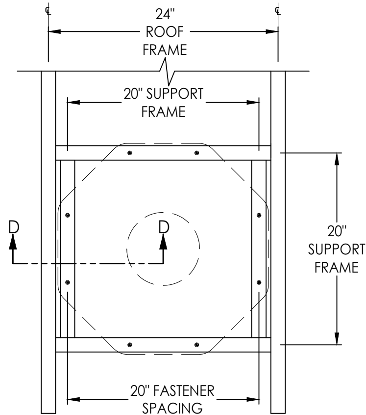
FRAMING DETAIL 10"
