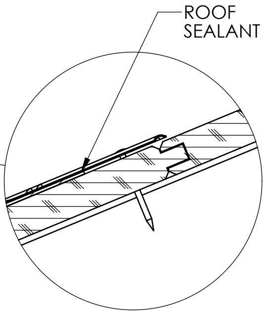
DETAIL C SCALE 1 : 2
