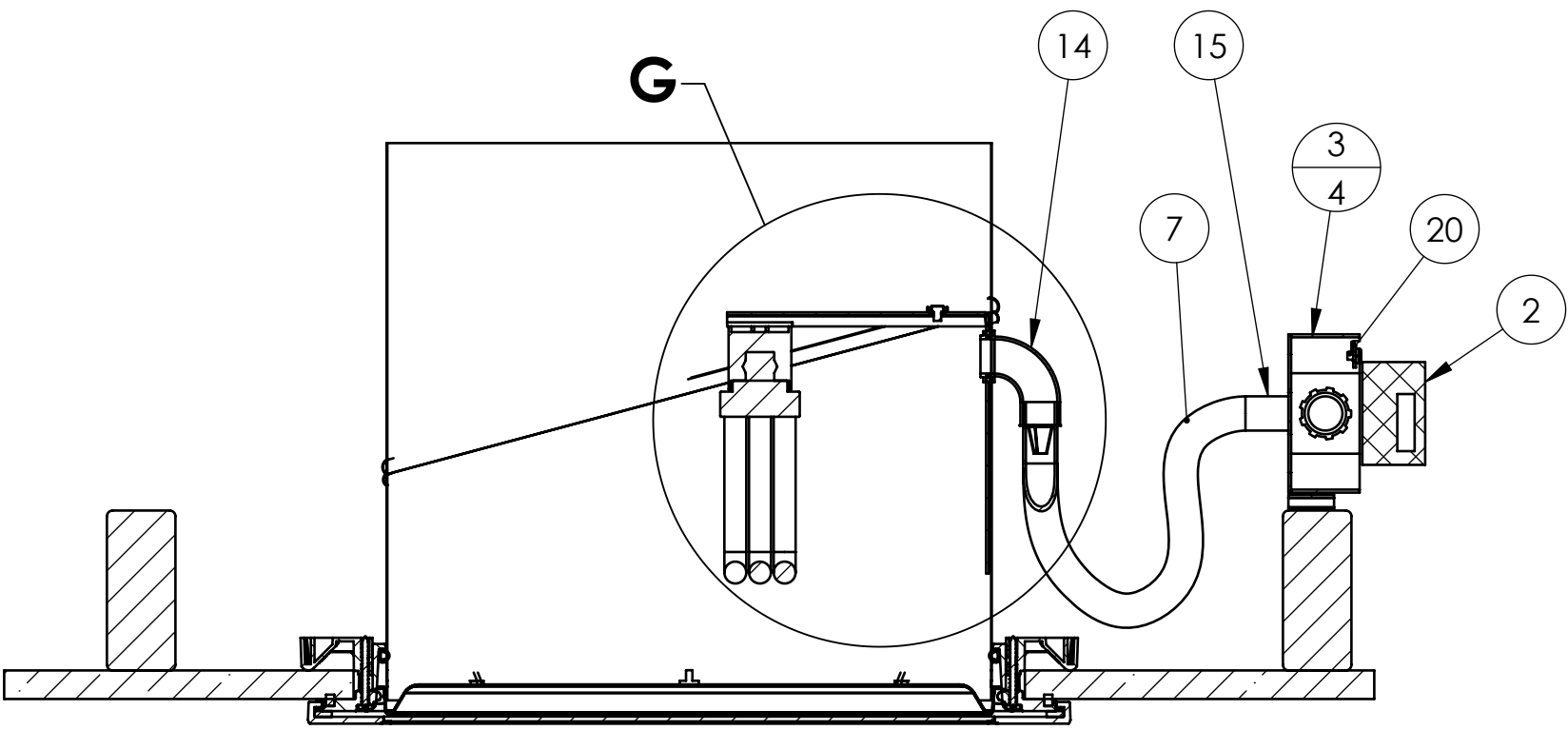
SECTION H-H
