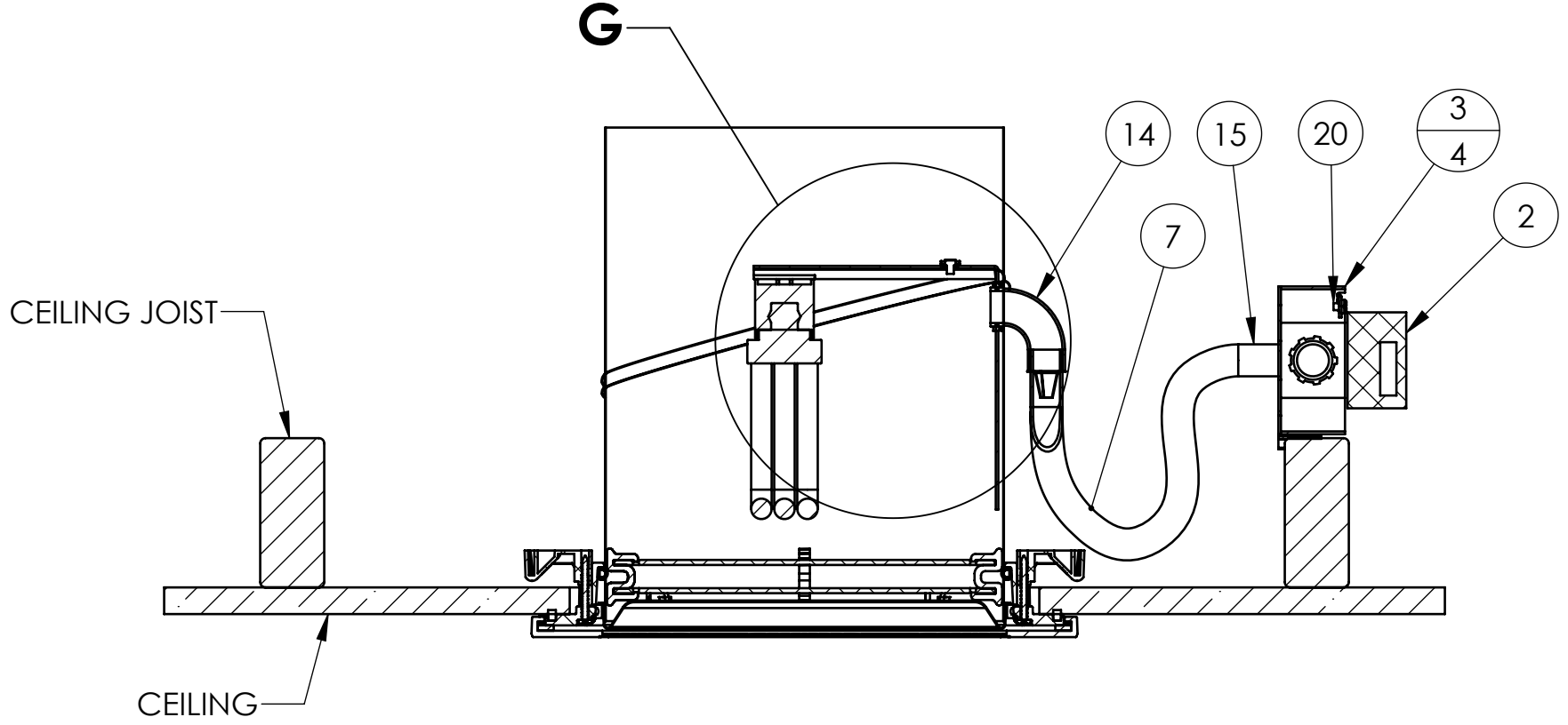
SECTION F-F
