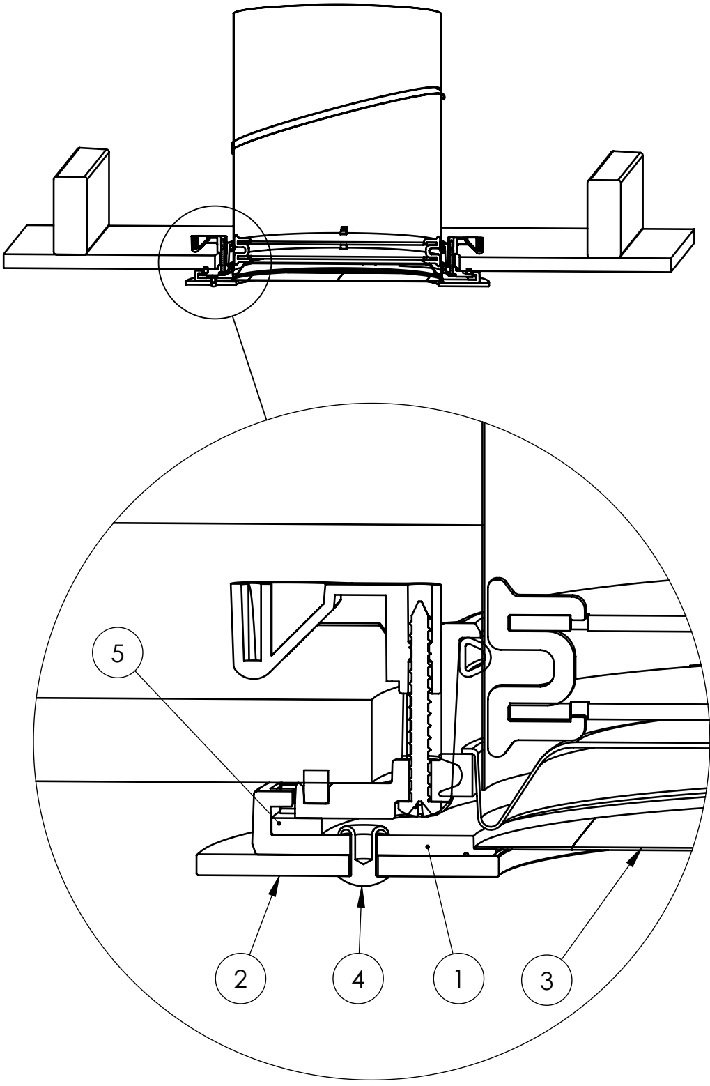
'OPTIVIEW' DIFFUSER ASSEMBLY
