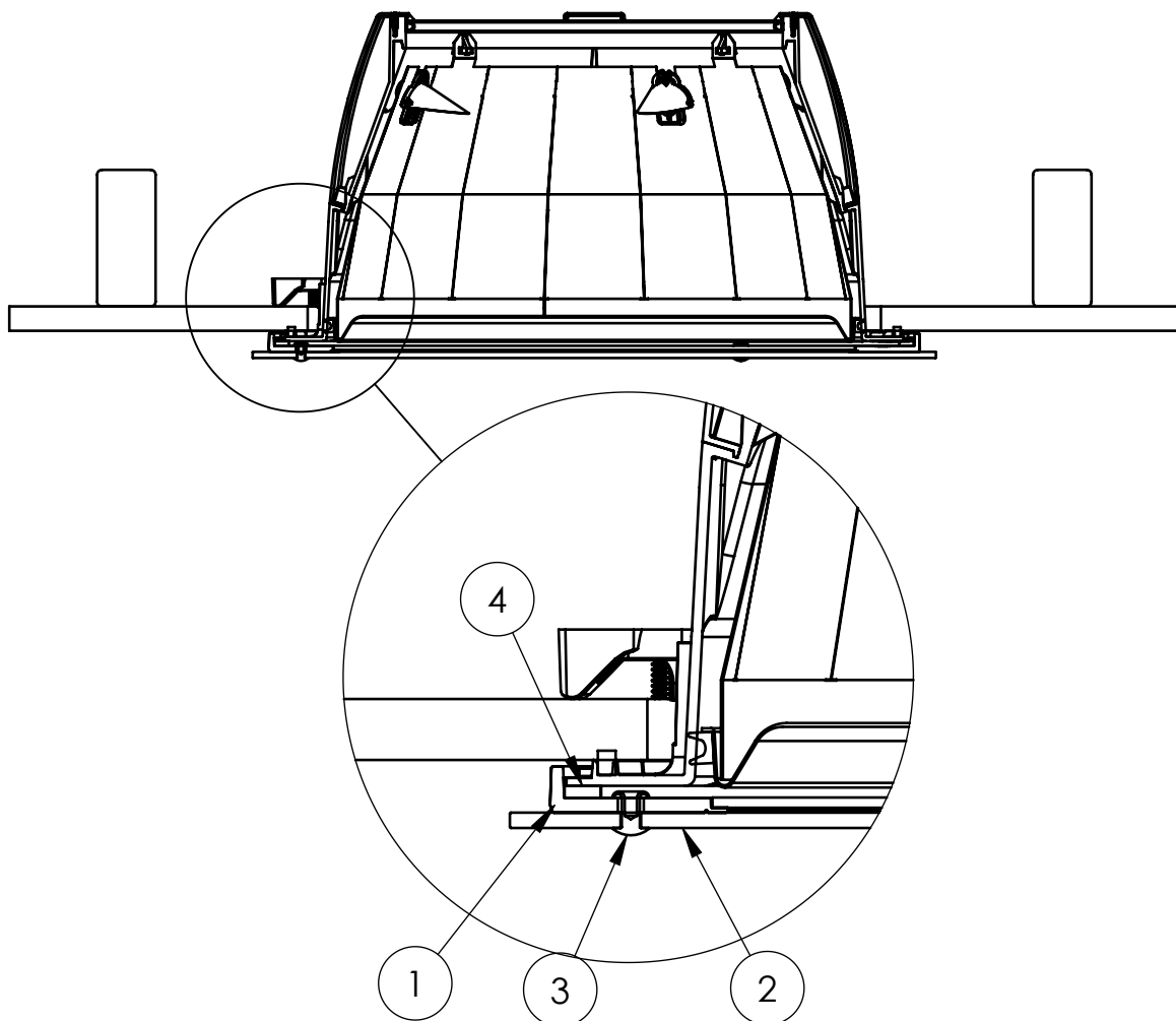
'JUST FROST' DIFFUSER ASSEMBLY
