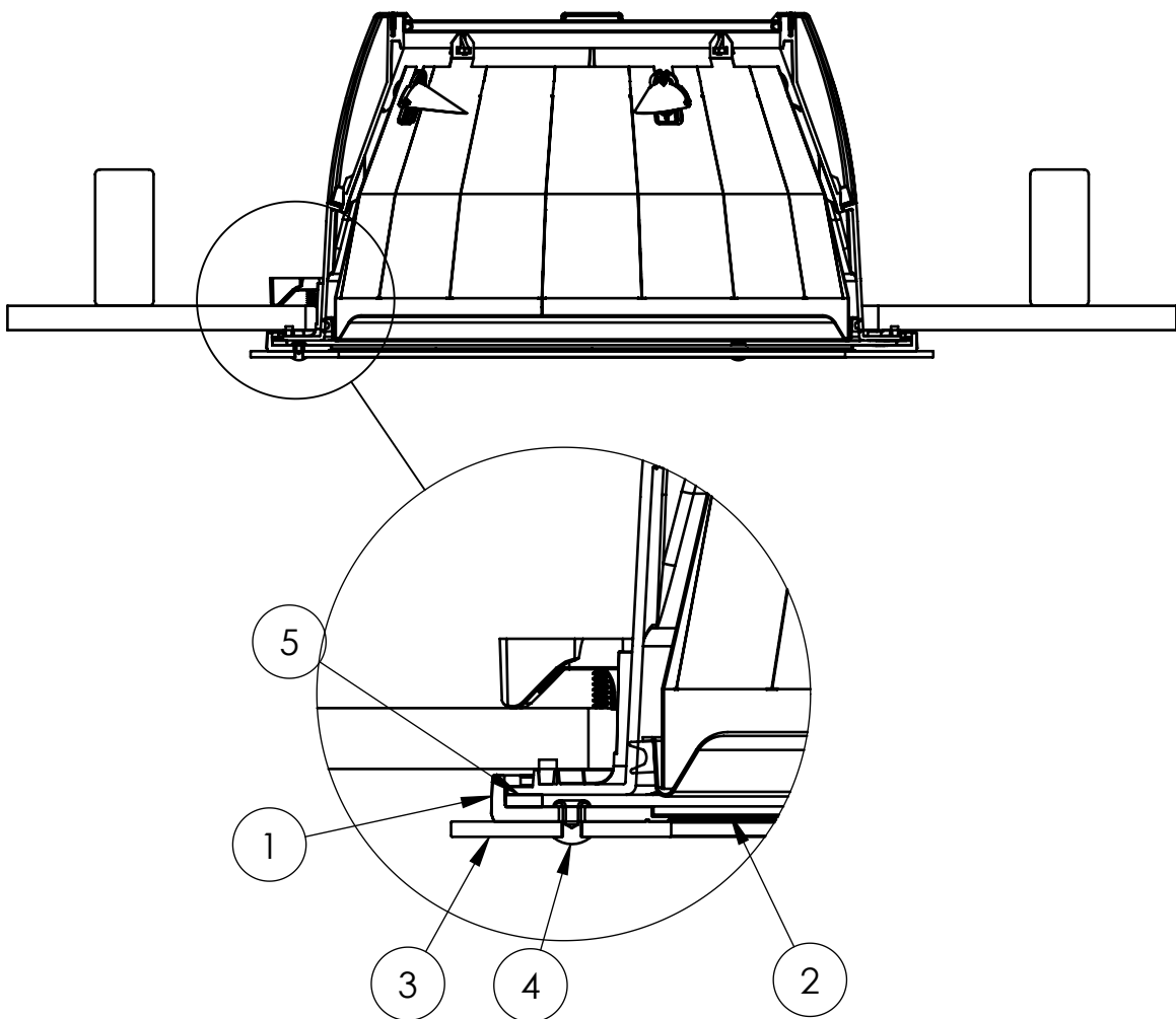
'OPTIVIEW' DIFFUSER ASSEMBLY
