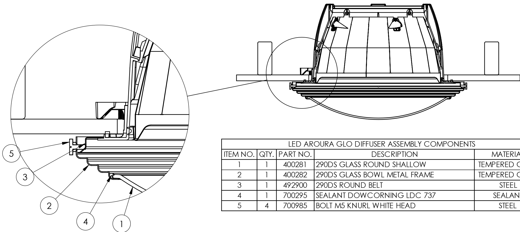
'AURORA GLO' DIFFUSER ASSEMBLY
