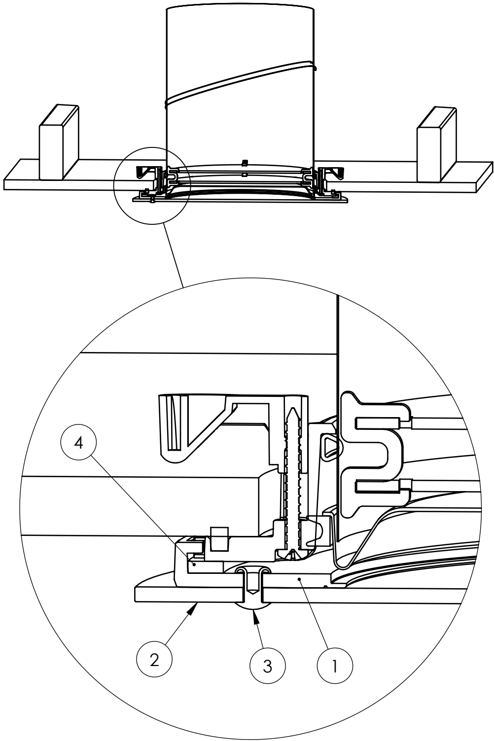
'JUST FROST' DIFFUSER ASSEMBLY
