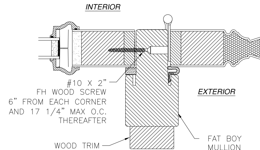
INSWING MULLION DETAIL WITH FAT BOY MULLION
