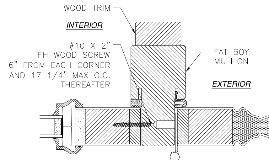
OUTSWING MULLION DETAIL WITH FAT BOY MULLION
