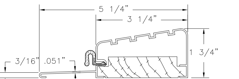
OUTSWING SILL
