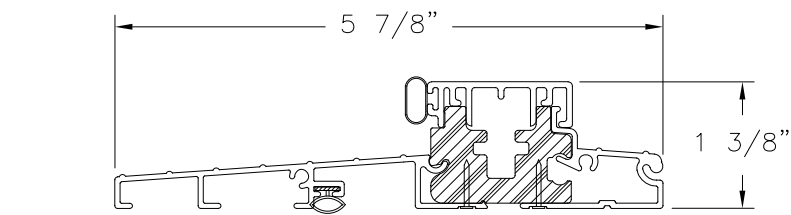
STANDARD OUTSWING SILL
