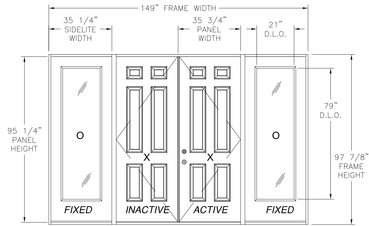
HERITAGE FIBERGLASS OPAQUE INSWING/OUTSWING DOUBLE DOOR W/SIDELITES EXTERIOR VIEW
