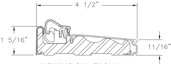
INSWING SILL ZA4565H
