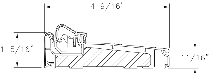
INSWING SILL ZA4565
