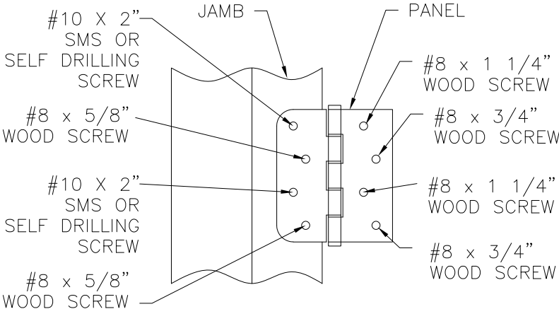
HINGE INSTALLATION DETAIL METAL STRUCTURE
