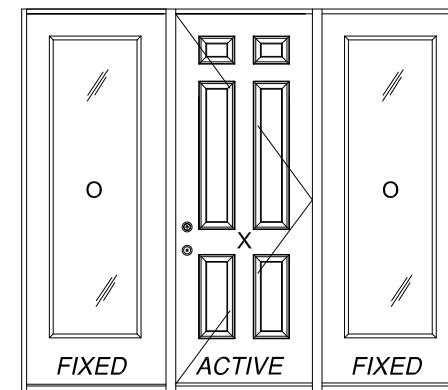
SINGLE W/SIDELITES EXTERIOR VIEW
