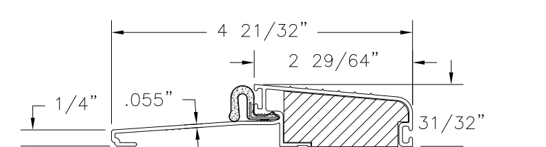
OUTSWING SILL
