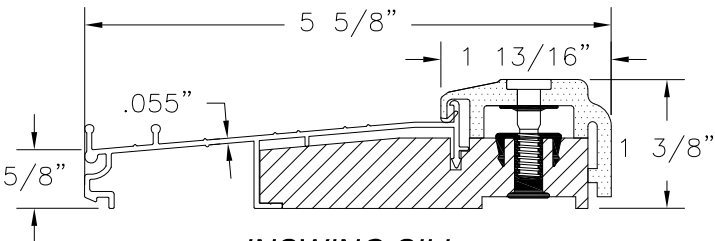
INSWING SILL
