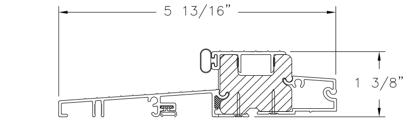
OUTSWING SILL
