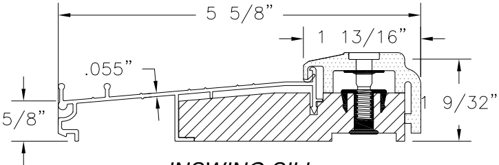
INSWING SILL
