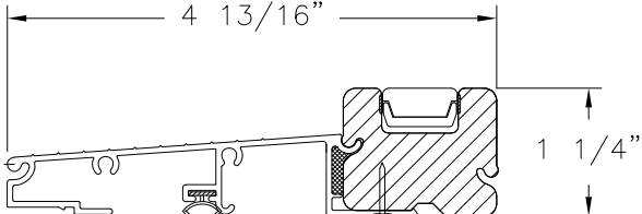
INSWING SILL
