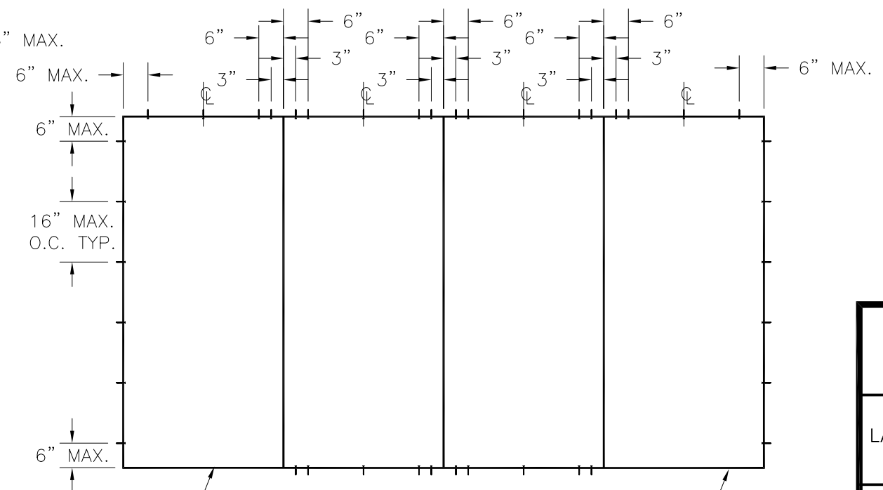
DOUBLE W/SIDELITES
