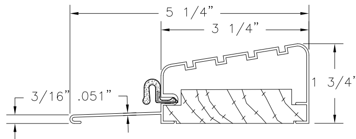
OUTSWING SILL
