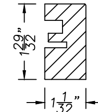
INTERIOR SILL TRIM (21)
