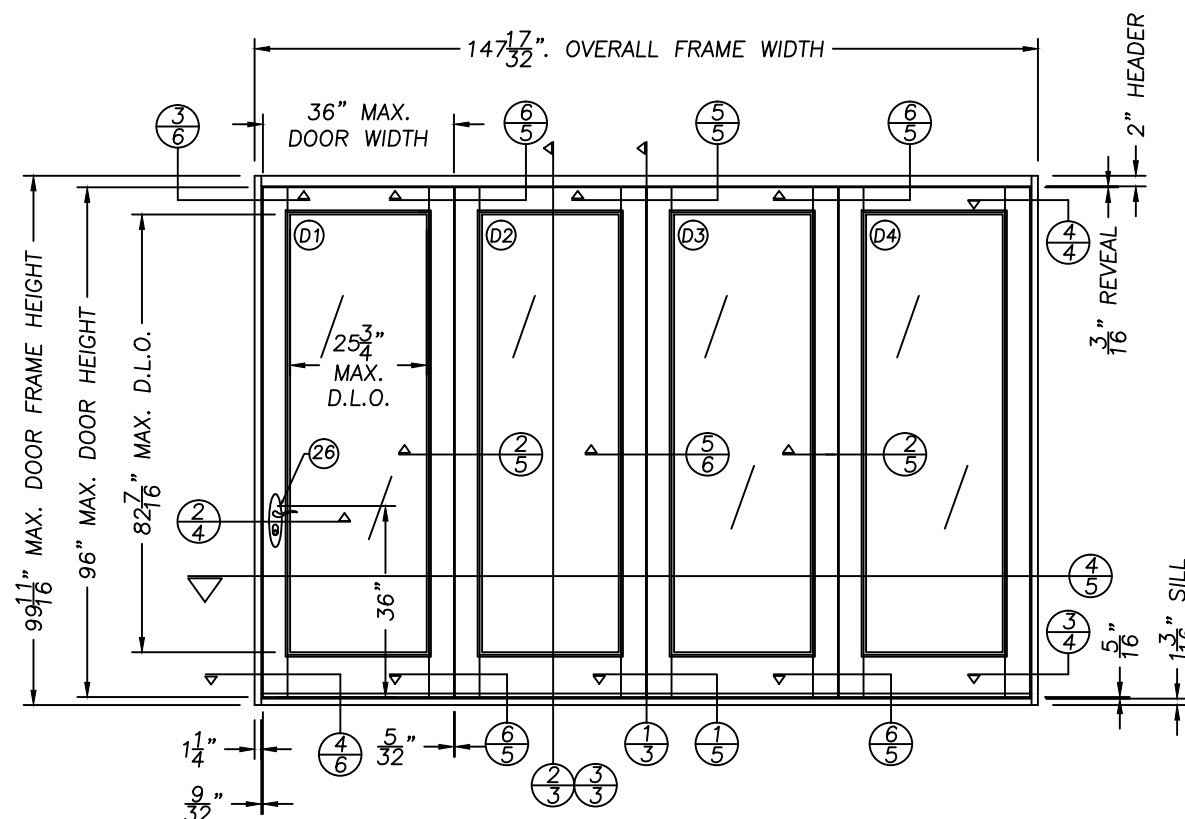
SYSTEM TYPE (4L) 4R MIRRORS 4L SYSTEM
