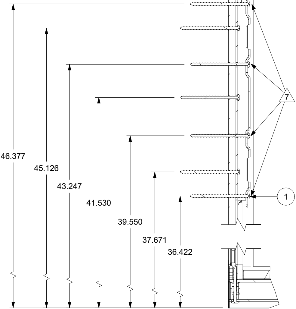
DETAIL A KEEPER SCREW PLACEMENT SCALE 1 : 3
