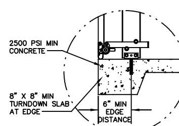
DETAIL H
