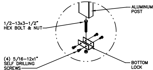
DETAIL G
