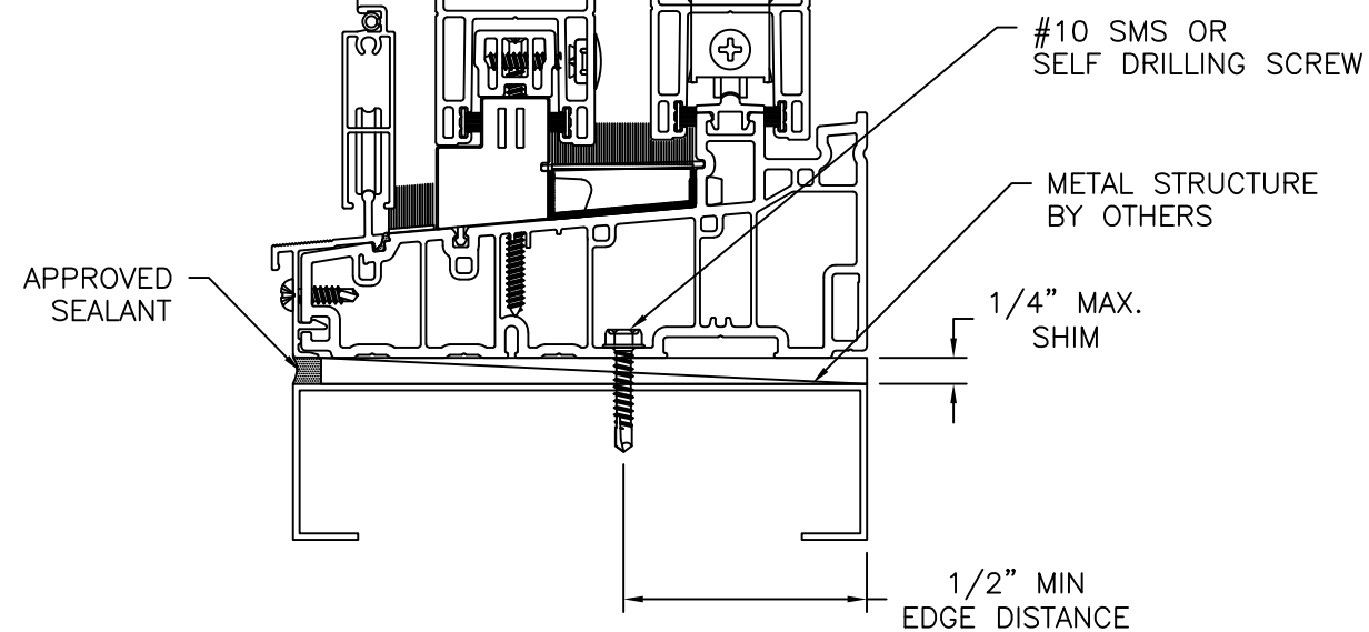
VERTICAL CROSS SECTION METAL STRUCTURE THROUGH FRAME INSTALLATION
