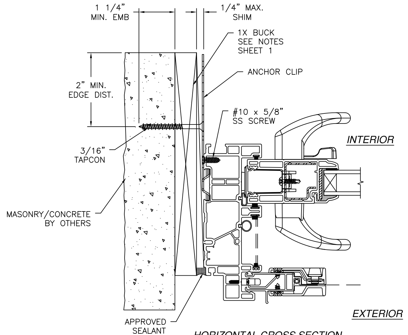
HORIZONTAL CROSS SECTION MASONRY/CONCRETE CLIP INSTALLATION
