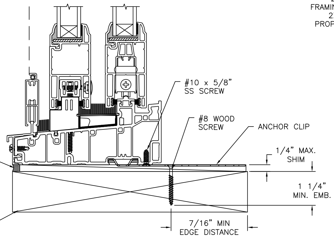
VERTICAL CROSS SECTION 2X BUCK/WOOD FRAMING CLIP INSTALLATION
