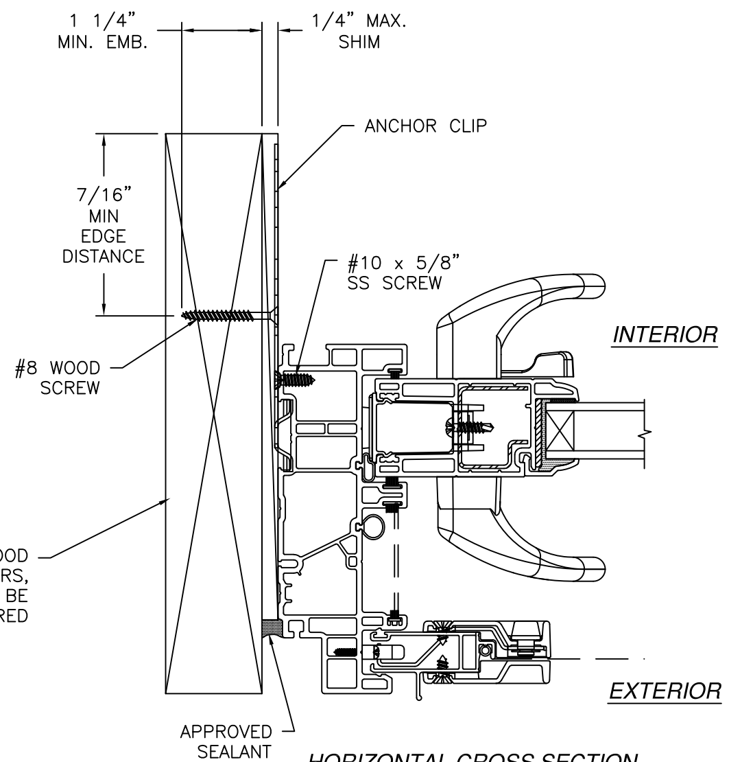
HORIZONTAL CROSS SECTION 2X BUCK/WOOD FRAMING CLIP INSTALLATION
