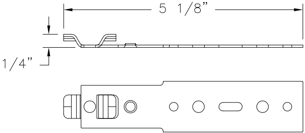
#9859 CLIP GALVANIZED STEEL .048" THICK
