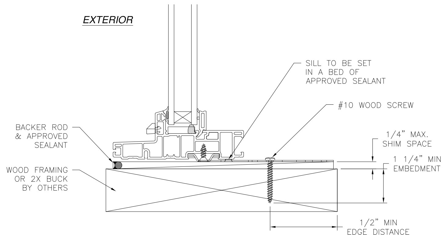
VERTICAL CROSS SECTION WOOD FRAMING OR 2X BUCK INSTALLATION JAMBS SIMILAR
