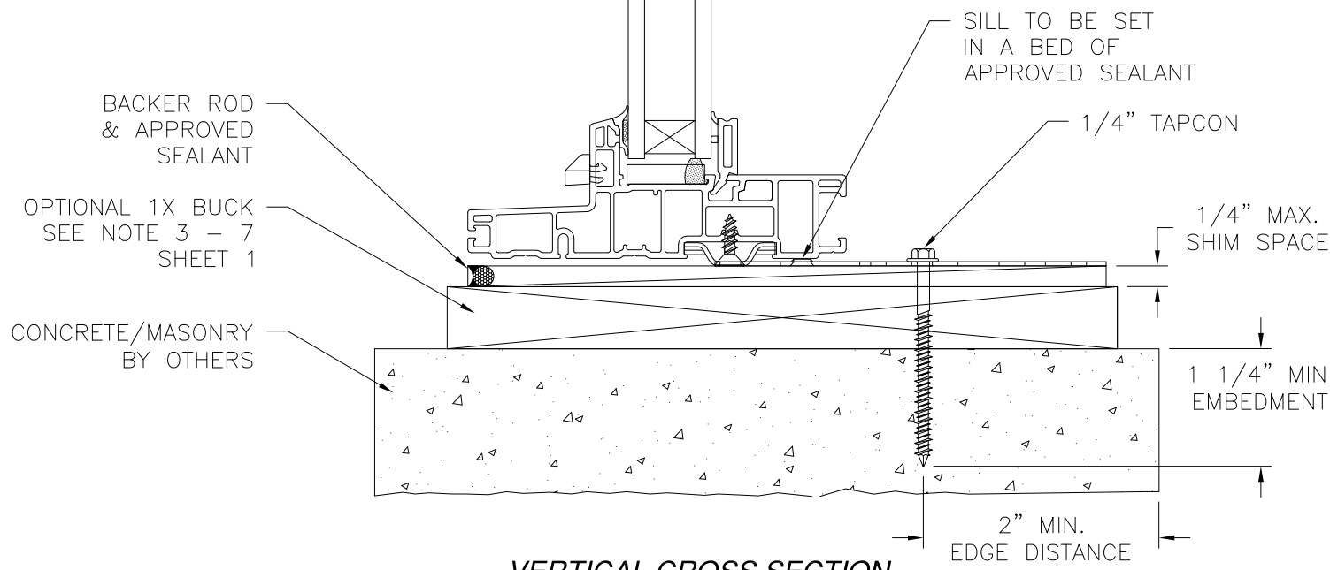
VERTICAL CROSS SECTION CONCRETE/MASONRY INSTALLATION JAMBS SIMILAR
