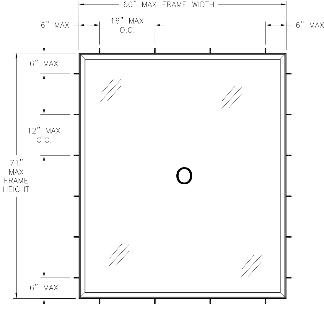
PRESTIGE 7110/7111/8110/8111 FIXED WINDOW EXTERIOR VIEW CLIP INSTALLATION
