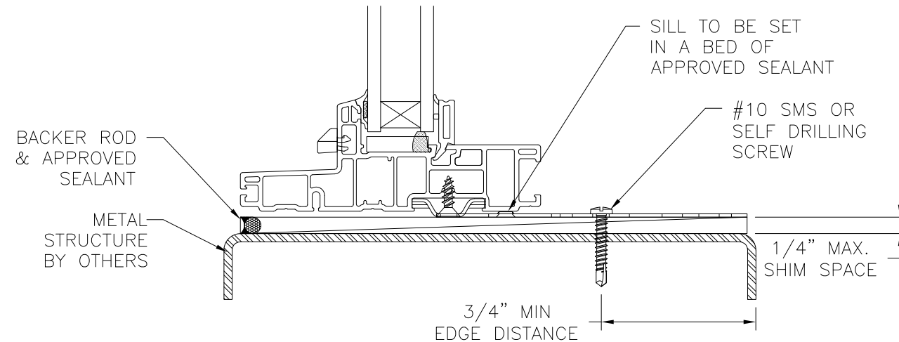
VERTICAL CROSS SECTION METAL STRUCTURE INSTALLATION JAMBS SIMILAR
