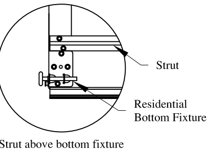
Strut above bottom fixture
