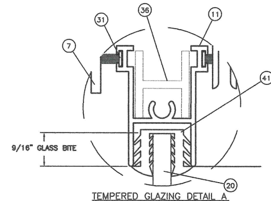
TEMPERED GLAZING DETAIL A
