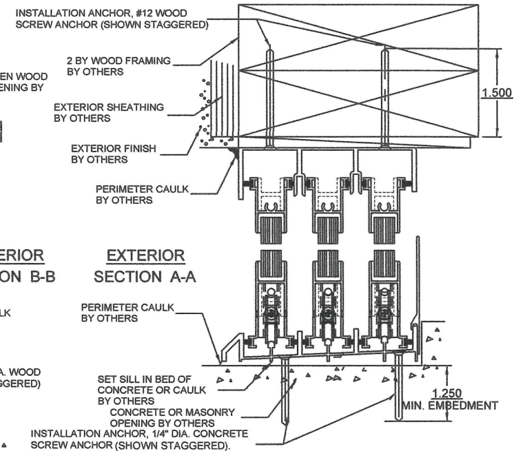
TYPICAL DETAIL AT 2 BY WOOD FRAMING
