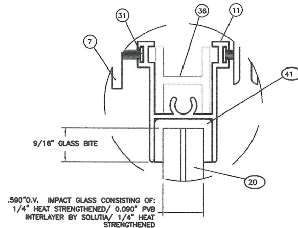
IMPACT GLAZING DETAIL A
