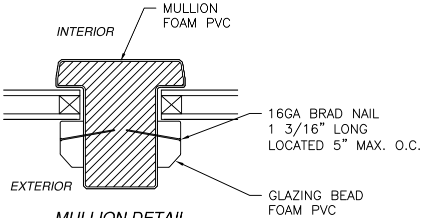
MULLION DETAIL
