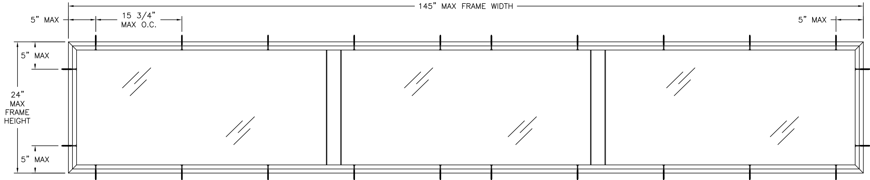
GTO 12020 GLAZED TRANSOM EXTERIOR VIEW
