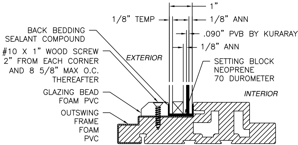
GLAZING DETAIL
