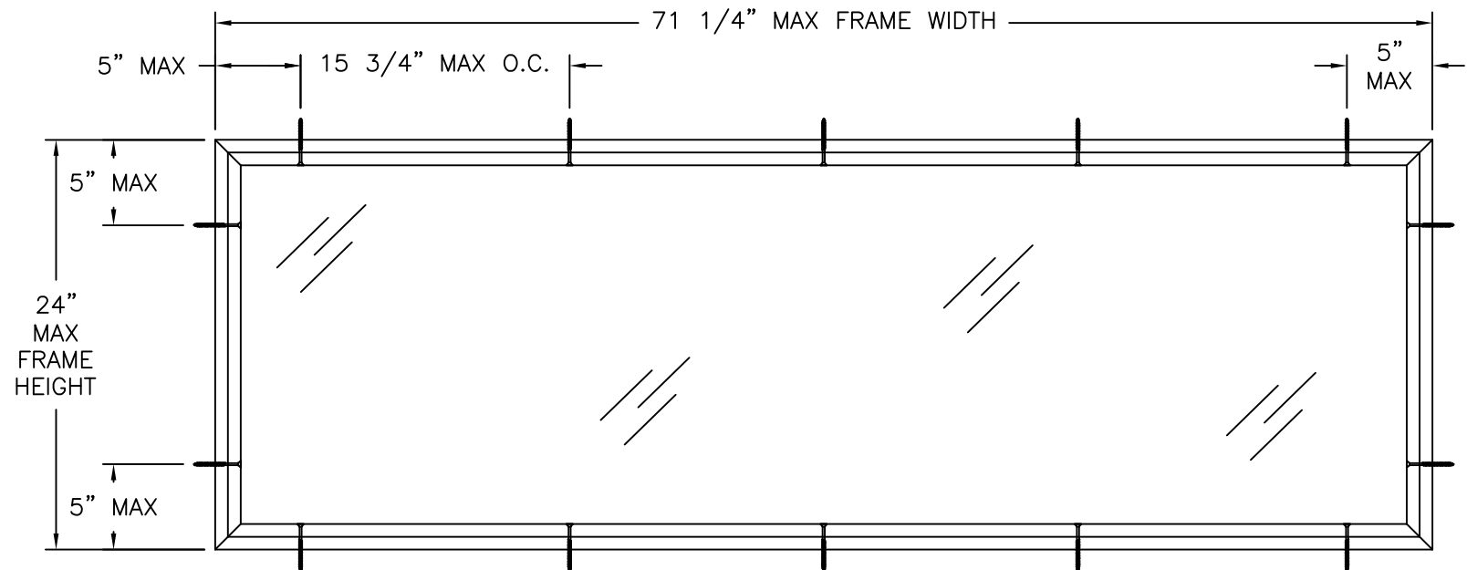
GTI 6020 IN-SWING TRANSOM - IMPACT EXTERIOR VIEW
