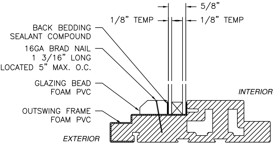
GLAZING DETAIL
