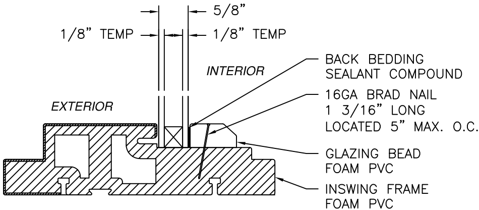
GLAZING DETAIL
